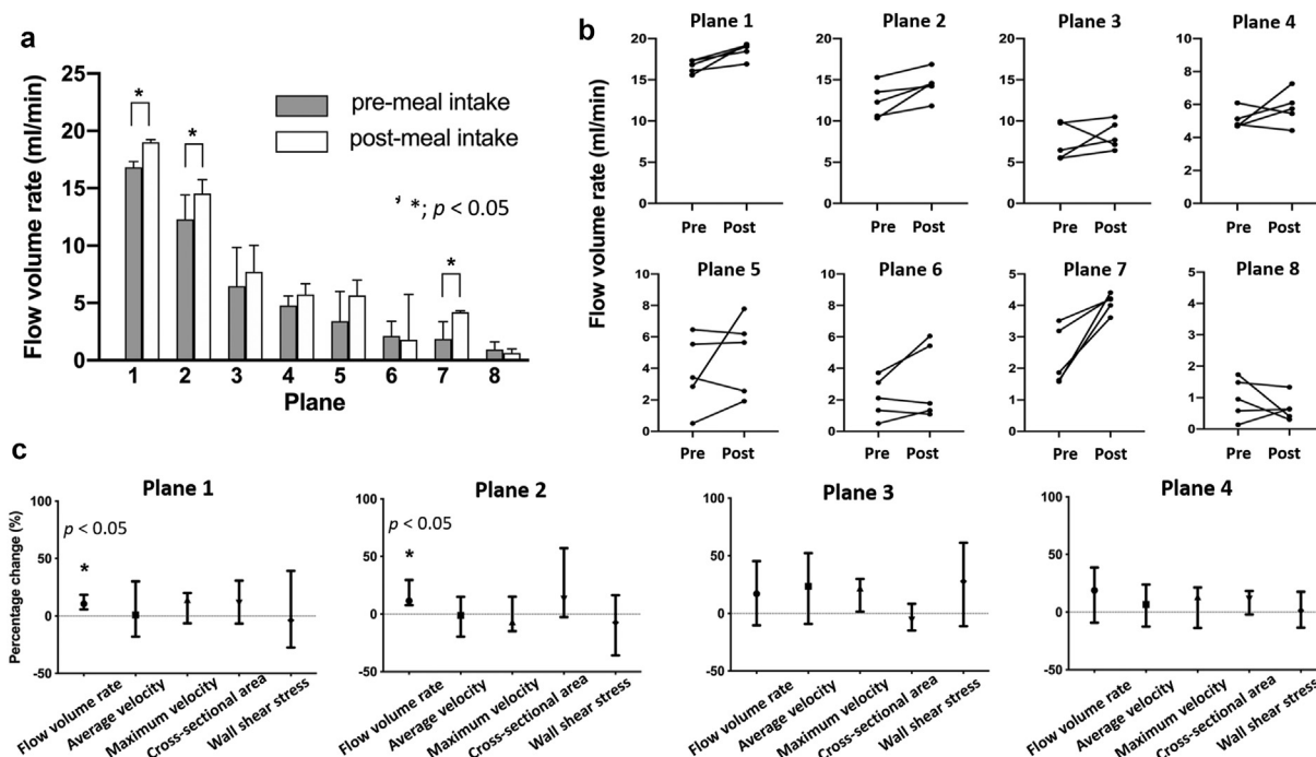
Figure 4 Changes in flow volume rate in response to a meal challenge for all eight analysis planes. (a) ( n = 5 ) Each bar represents the IQR. Flow volume rate increased significantly in planes 1 ( p = 0.02 ), 2 ( p = 0.03 ) and 7 ( p = 0.01 ). The graphs represent the changes in flow volume rate in all eight planes in all five rats (b). Percentage changes for all measurements in four planes (c). (* = significant difference compared to data taken before the meal challenge, p < 0.05 )
