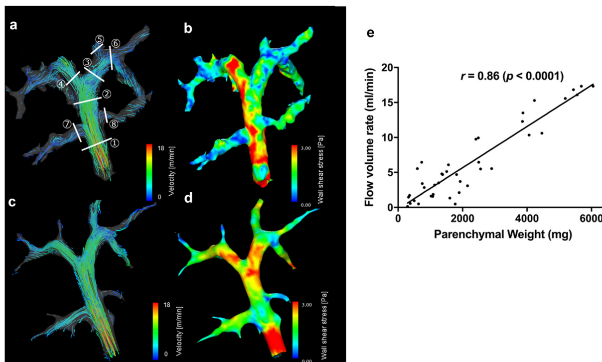
Figure 3 Assessment of PV tributaries by 3D PC-MRI. Representative data of the streamlines (a) and WSS (b) prior to meal intake were mapped out, overlaid on a PV tree image. The planes of assessment are shown: 1, the main PV; 2, the branch feeding the middle and left lateral; 3, the branch feeding the left median and left lateral lobes; 4, the branch to the right median lobe; 5, the branch to the left median lobe; 6, the branch to the left lateral lobe; 7, the branch to the right lobe; 8, the branch to the caudate lobe. The streamlines (c) and WSS mapping (d) in the same animal after meal intake are shown as an indicator of PV flow changes in response to meal intake. The flow volume rate of each PV branch and the corresponding parenchymal weight are plotted, showing a strong correlation between the two parameters (a correlation coefficient of 0.86, p < 0.0001 ) (e)
