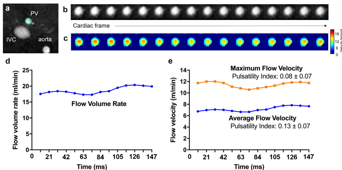
Figure 1 Assessment of the main PV using respiratory- and cardiac-gated 2D cine PC-MRI. An MR angiography image (a) shows the plane of assessment, which includes the PV, IVC, and aorta. Representative magnitude images (b) and velocity images (c) of the main PV are shown as sequential images during one cardiac cycle with a temporal resolution of 10.5 ms. Hemodynamic changes during a single cardiac cycle are shown, revealing flow volume rates (d) and maximum and average flow velocities (e). PV, portal vein; IVC, inferior vena cava; 2D cine PC-MRI, two-dimensional phase-contrast MRI
