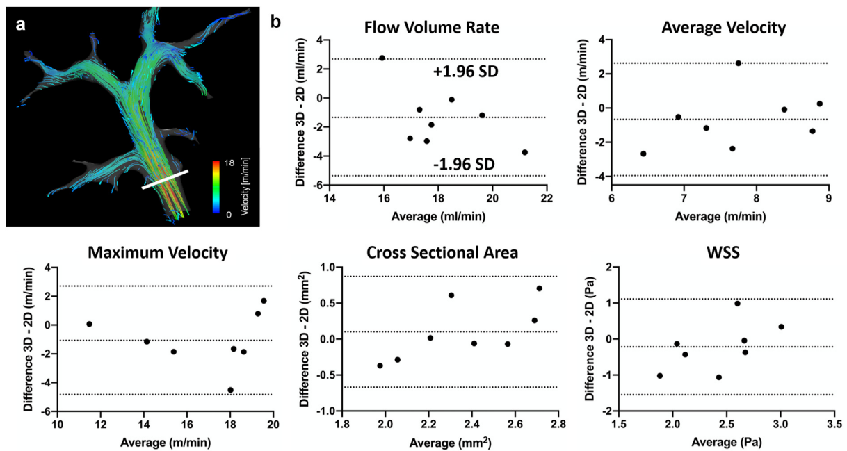
Figure 2 Assessment of the main PV using 3D PC-MRI. (a) The streamlines are visualized as color-coded lines, overlaid on a PV tree image obtained from time-of-flight MR angiography. The plane for flow assessment is indicated by the white line. (b) Bland–Altman plot of data obtained by 2D cine PC-MRI and that obtained by 3D PC-MRI for flow volume rate, average and maximum velocities, cross-sectional area, and WSS. The dashed lines indicate bias, lower and higher limits of agreement. 2D cine PC-MRI, two-dimensional phase-contrast MRI; 3D PC-MRI, three-dimensional phase-contrast MRI; PV, portal vein; WSS, wall shear stress. Each bar represents the IQR
