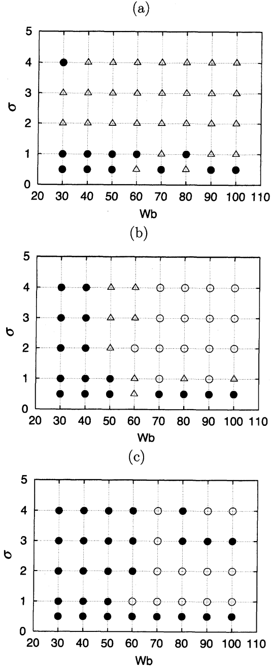
Figure 6: Classifications of the breakup profiles in the parameter space Wb and \sigma when Re = 10 , where \triangle , \circ and \bullet , respectively, denote the cases when the breakup is due to disintegration, ballooning and closing of the annular phase: (a) n = 0.2 , (b) n = 1 and (c) n = 1.8 .
