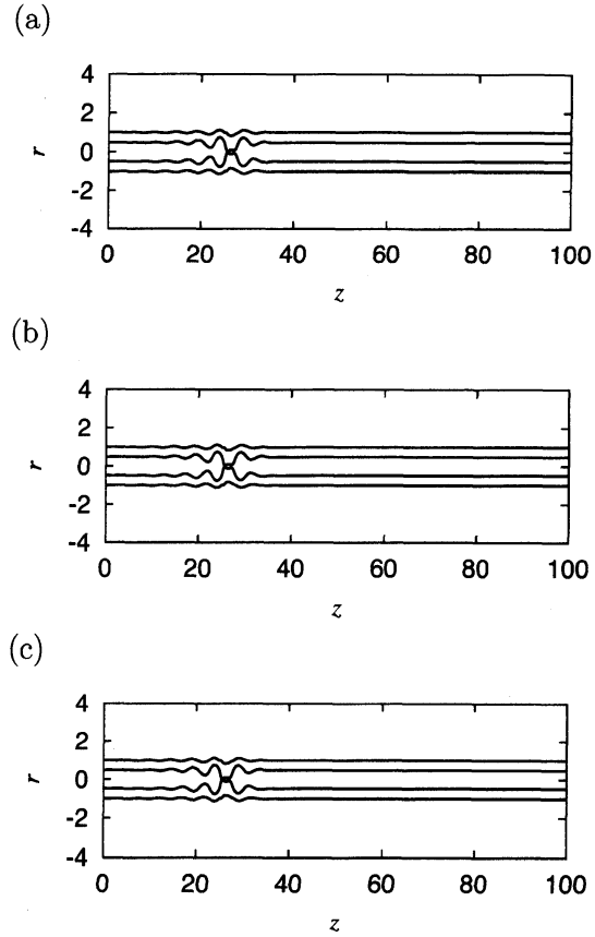
Figure 3: Breakup profiles for different n when \sigma = 2.6 , \text{Re} = 354 and \text{Wb} = 47.9 ; (a) n = 0.2 ( t_b = 28.75 , z_b = 25.80 , \omega_c = 1.35 ), (b) n = 1 ( t_b = 28.75 , z_b = 25.80 , \omega_c = 1.35 ) and (c) n = 1.8 ( t_b = 28.80 , z_b = 25.80 , \omega_c = 1.35 ).
