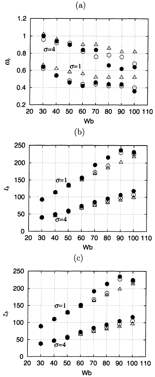
Figure 7: Variations of \omega_c , t_b and z_b for Wb when \sigma = 1 and 4 and Re = 10 , where \triangle : n = 0.2 , \circ : n = 1 and \bullet : n = 1.8 .
