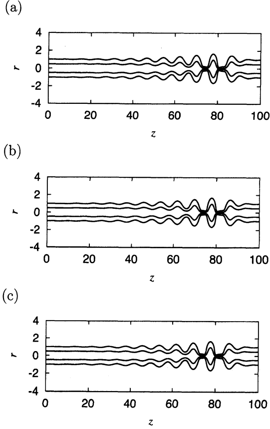
Figure 2: Breakup profiles for different n when \sigma = 0.1 , \text{Re} = 354 and \text{Wb} = 47.9 ; (a) n = 0.2 ( t_b = 85.90 , z_b = 80.60 , \omega_c = 0.80 ), (b) n = 1 ( t_b = 85.95 , z_b = 80.60 , \omega_c = 0.80 ) and (c) n = 1.8 ( t_b = 85.95 , z_b = 80.60 , \omega_c = 0.78 ).
