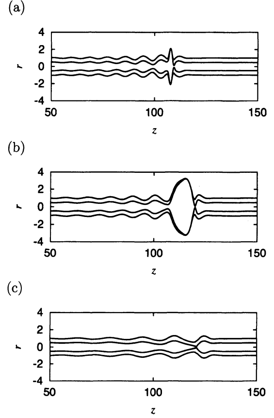
Figure 5: Typical three breakup profiles - disintegration, ballooning and closing- for different n when \sigma = 2.6 , \text{Re} = 10 and \text{Wb} = 80 : (a) n = 0.2 ( t_b = 111.95 , z_b = 109.40 , \omega_c = 0.72 ), (b) n = 1 ( t_b = 122.20 , z_b = 120.00 , \omega_c = 0.58 ) and (c) n = 1.8 ( t_b = 125.80 , z_b = 120.60 , \omega_c = 0.40 ).
