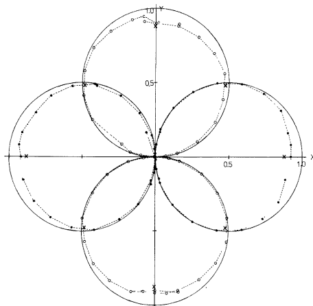
Fig. 10 Directional diagram showing response of ultra-sonic current meter employed.
