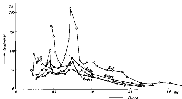
Fig. 2 Acceleration spectrum.
