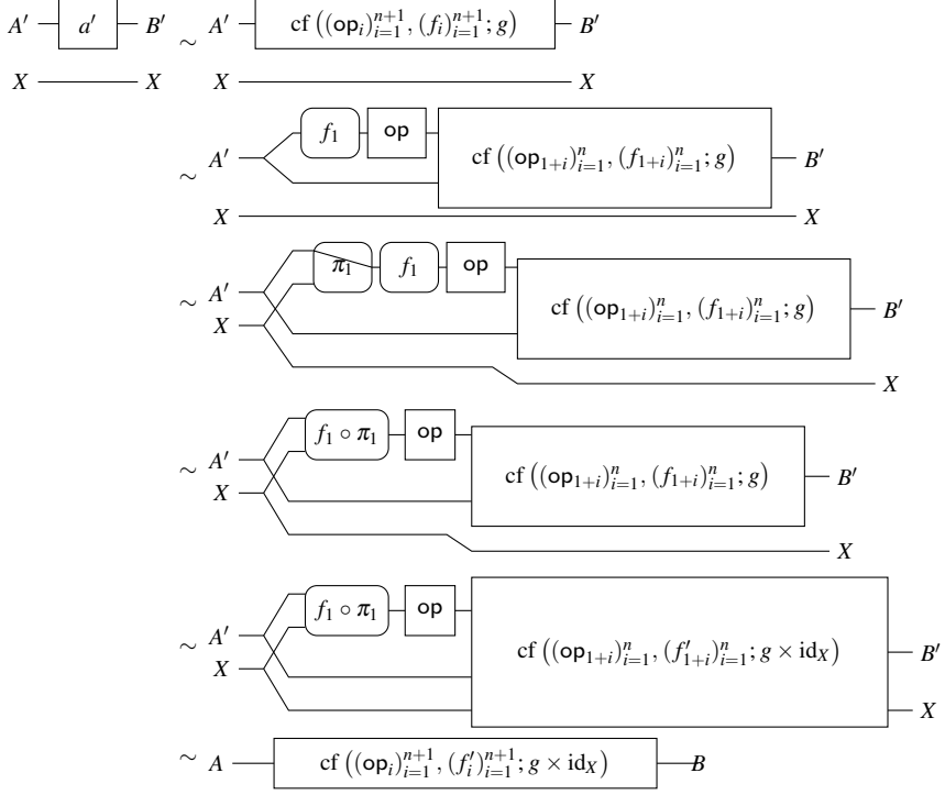
Fig. 9. In case a = \text{first}_X(a') and a' \sim \text{cf}((\text{op})_{i=1}^{n+1}, (f_i)_{i=1}^{n+1}; g) .
