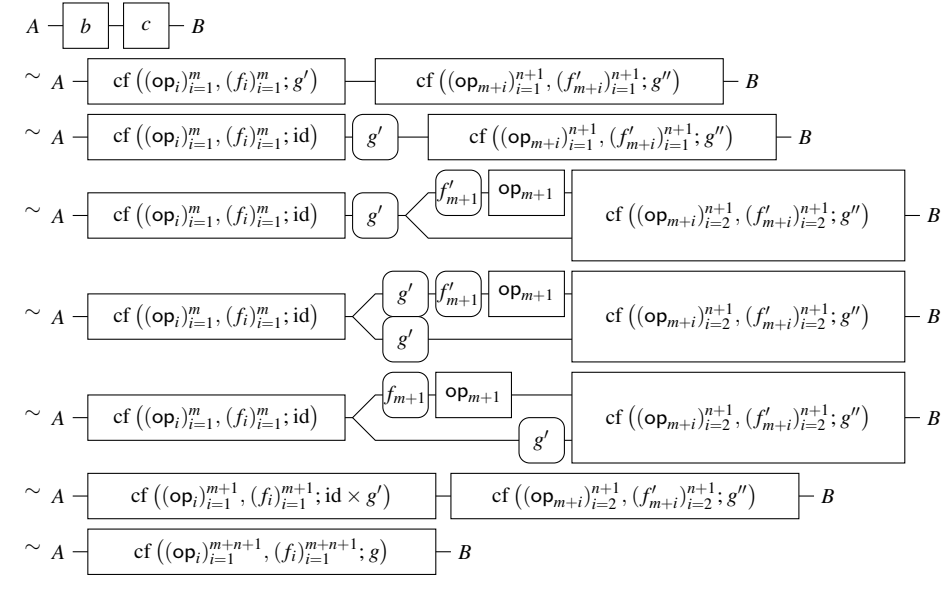
Fig. 10. In case a = b \gg c and c \sim \text{cf} \left( (\text{op}_i)_{i=1}^{n+1}, (f_i')_{i=1}^{n+1}; g'' \right) .
