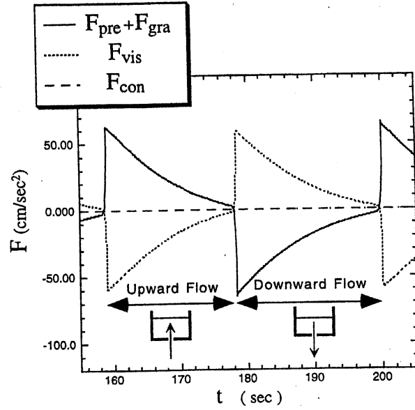
Figure 7: Time-dependent change in the individual components of the force needed to induce acceleration in fluid flow. F_{con} is the convection term, F_{pre} is the pressure term, and F_{vis} is the viscosity term, and F_{gra} is the gravity term.
