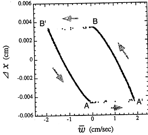
Figure 6: Numerical simulation of the limit-cycle behavior in the saline oscillator shown as \Delta x vs. \bar{w} , where \Delta x = x - H_{eq}(n) and \bar{w} is the average velocity at the orifice. The interval between the data points is 0.1 sec.
