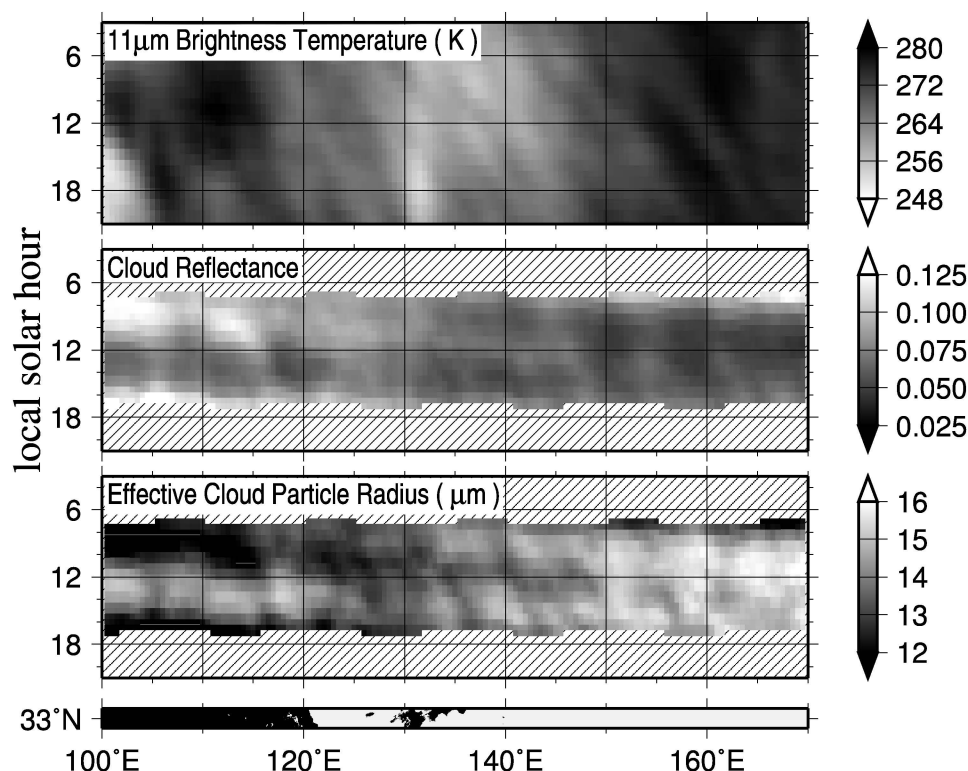
Fig. 3 Longitude-local solar hour cross section diagram in 33°N showing 11 \mu m brightness temperature, cloud reflectance, effective radius of cloud particle and land-sea distribution as a monthly mean from 24 June 2007.
