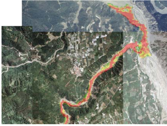
Fig.9 The simulation result – Nantou072, the depth in detention basin condition case
