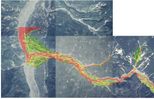
Fig.3 The simulation result — Nantou026, the depth in natural condition case
