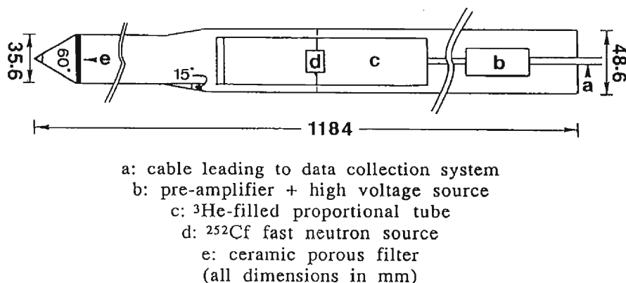
Fig. 6. The schematic diagramme of the Neutron Moisture Cone Penetrometer.
