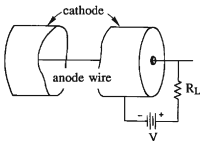
Fig. 4. Basic elements of proportional counter. The outer cathode provides a vacuum tight enclosure for the fill gas. The output pulse is developed across the load resistance (Knoll 15 ).
