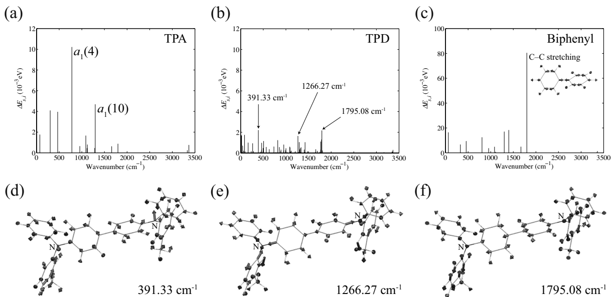
Figure 2.6: Contribution to \Delta E_s from each mode for various cations: (a) TPA; (b) TPD; (c) Biphenyl. Various vibrational modes of TPD: (d) 391.33 \text{cm}^{-1} ; (e) 1266.27 \text{cm}^{-1} ; (f) 1795.08 \text{cm}^{-1} .
