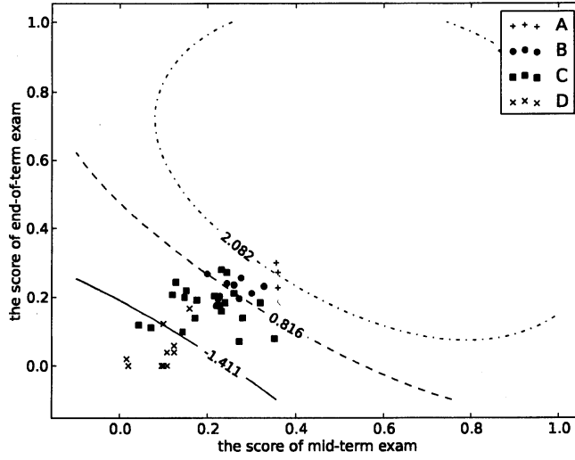
FIGURE 2. Classification by (\tilde{S}_1) with the Gaussian kernel
