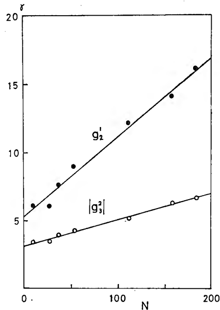
Fig. 3. Correlation between the relative sunspot number N and g_2^1 or g_3^2 .
