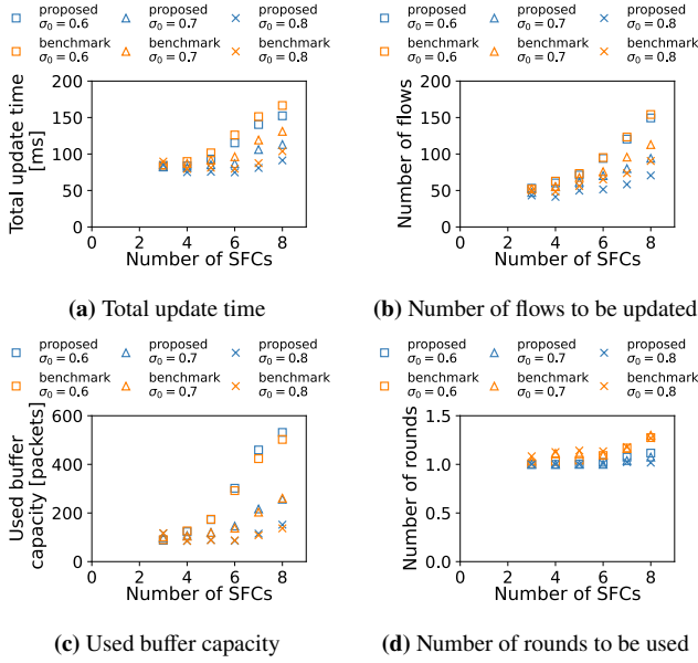
Fig. 8: Results when buffer capacity is c^{\text{buffer}} = 10000 [packets] in NSFNET.
