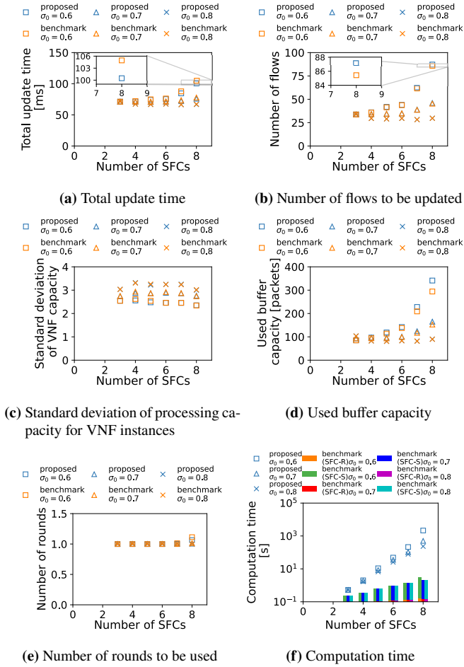
Fig. 5: Results when buffer capacity is c^{\text{buffer}} = 10000 [packets] in 8-node network.
