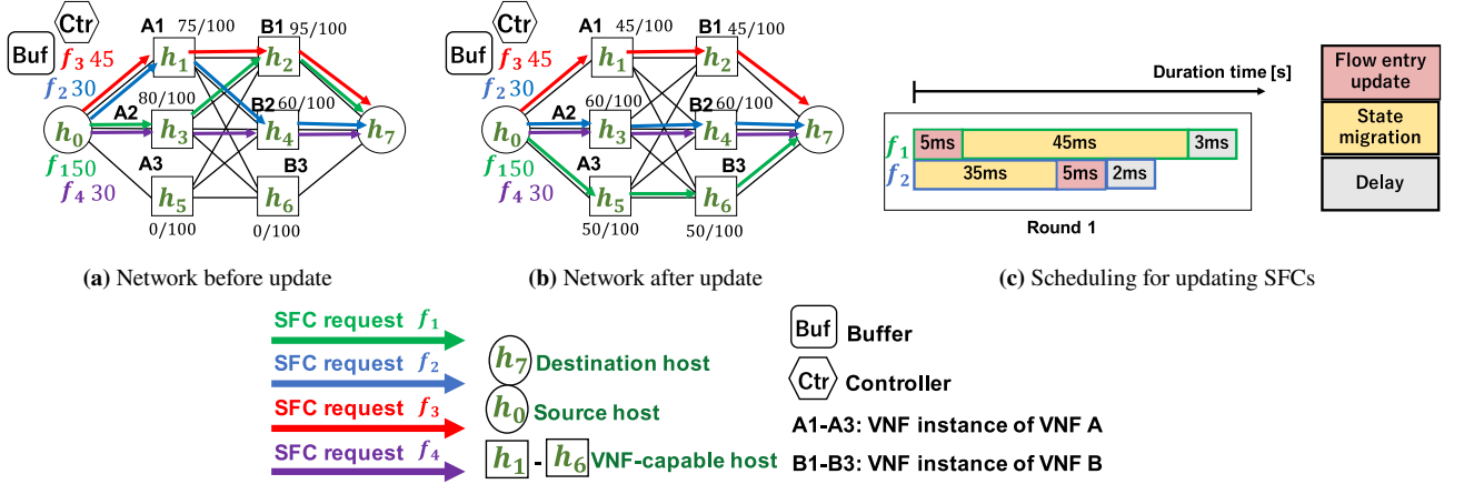
Fig. 3: Example of determination of SFCs to be updated, their routes, and update scheduling for multiple SFCs.
