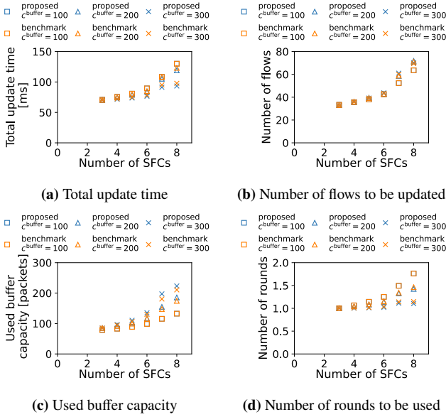
Fig. 6: Results when threshold of capacity utilization ratio is \sigma_0 = 0.6 in 8-node network.
