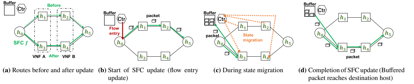
Fig. 2: Example of SFC update procedure by proposed model.
