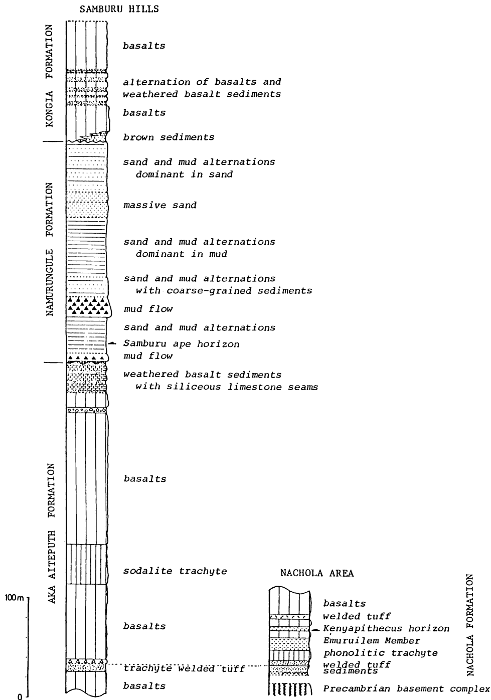
Fig. 4. Composite columnar sections of the Nachola, Aka Aiteputh, Namurungule and Kongia Formations.
