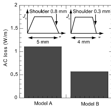
Fig. 3 Calculated AC loss of 2 layer cables: Model A is a cable composed by 5 mm wide conductors with 0.8 mm shoulders and Model B is 4 mm wide conductors with 0.3 mm shoulders.
