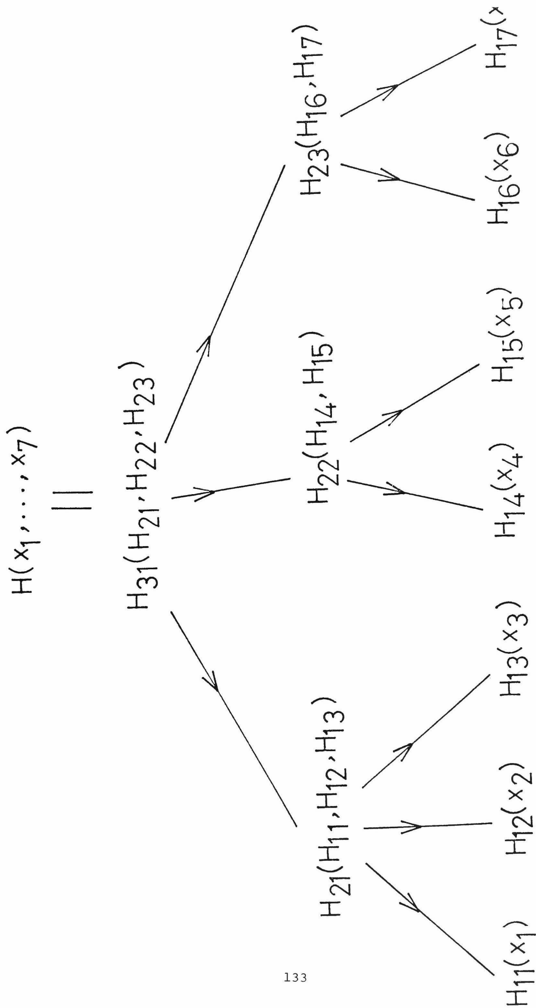
Fig. 7.2. Disjoint decomposition
