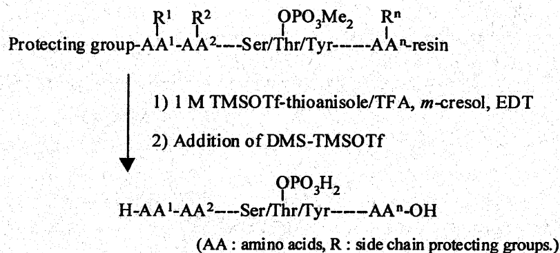
Figure 1. General deprotection scheme for the synthesis of phosphopeptides.
