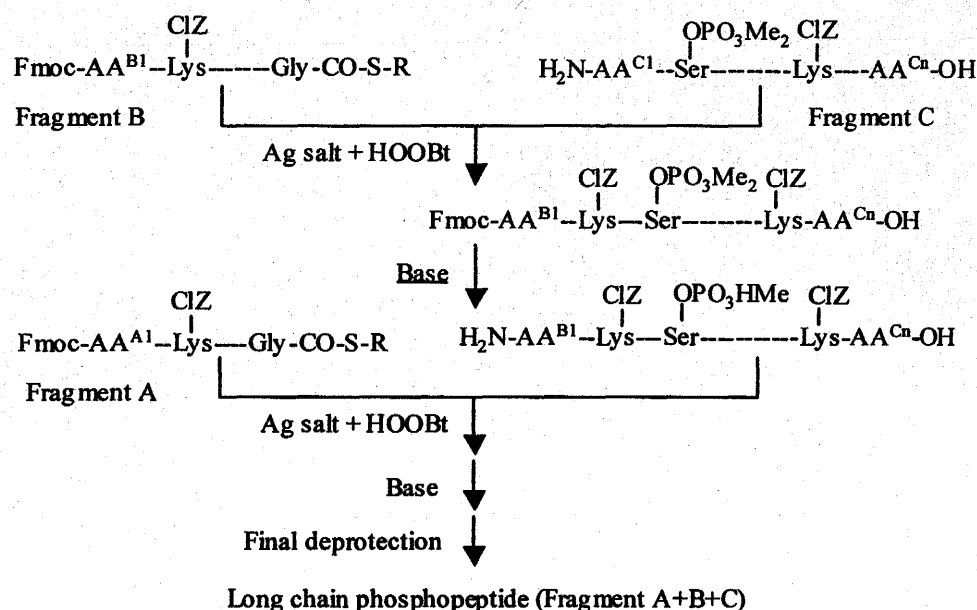
Figure 3. New synthetic methodology for long chain phosphopeptide.
