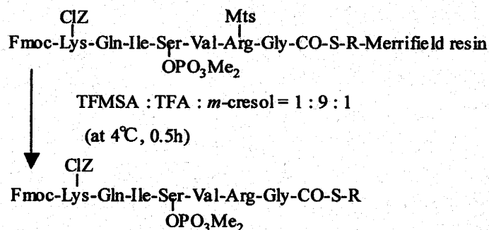
Figure 2. Synthesis of protected phosphopeptide fragment using High TFMSA.
