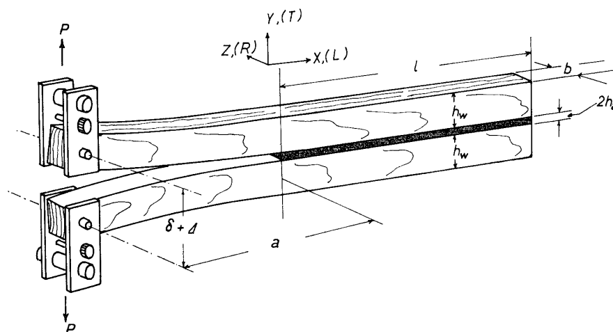
Fig. 1. Double Cantilever Beam (DCB) specimen with thick adhesive alyer. a : crack (beam) length, l : glue line length, h_w : depth of beam, b : thickness of specimen, 2h_a : thickness of glue line, \Delta = 2h_a + h_w , P : load, \delta : deflection.
