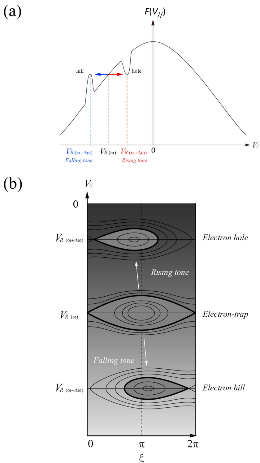
Figure 1. (a) Formation of an electron hole due to a rising tone element and an electron hill due to a falling tone element in the reduced velocity distribution function F(v_{||}) of energetic electrons at the equator and (b) the corresponding variations of g(v_{||}, \zeta) in velocity phase space (v_{||}, \zeta) .
