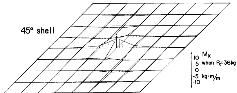
Fig. 23. The distribution of the bending moment M_x of the orthotropic cylindrical shells under a central concentrated load P_c . See Fig. 22.
