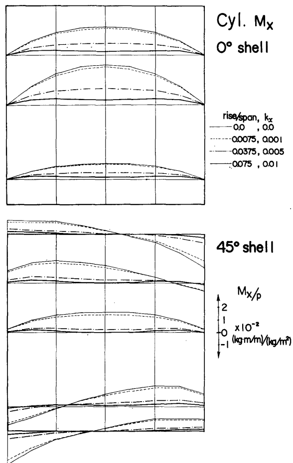
Fig. 13. Effect of the curvature on the bending moment of the orthotropic cylindrical shells under uniform pressure. See * in Fig. 7. When the case **** in Table 2, the unit of the scale is \times (\text{kg} \cdot \text{m}/\text{m})/(\text{kg}/\text{m}^2) .
