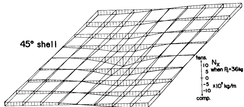
Fig. 24. The distribution of the membrane force N_x of the orthotropic cylindrical shells under a central concentrated load P_c . See Fig. 22.
