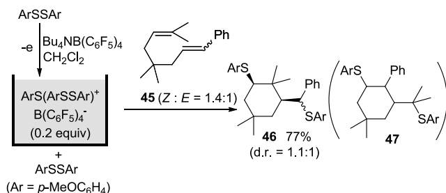
Scheme 15. \text{ArS(ArSSAr)}^+ \text{B(C}_6\text{F}_5)_4^- initiated addition of \text{ArSSAr} 10 to dienes via intramolecular C-C bond formation.
