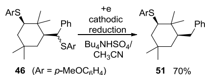
Scheme 17. Electroreductive removal of benzylic \text{ArS} from 35 product 46 (Ar = p -MeOC 6 H 4 ).
