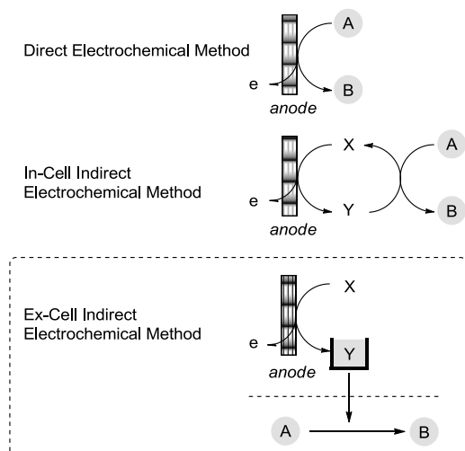
Scheme 1. Classification of electrochemical methods.
