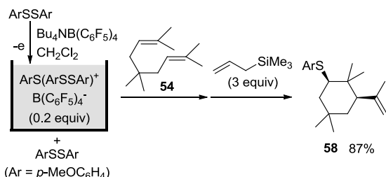
Scheme 20. The reaction of 54 with a catalytic amount of 65 \text{ArS(ArSSAr)}^+ \text{B(C}_6\text{F}_5)_4^- followed by adding allyltrimethylsilane (Ar = p -MeOC 6 H 4 ).
