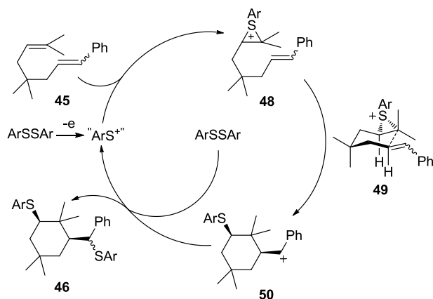
Scheme 16. Mechanism of “ \text{ArS}^+ ” ( = \text{ArS(ArSSAr)}^+ ) initiated 20 addition of \text{ArSSAr} to dienes via intramolecular C-C bond formation.
