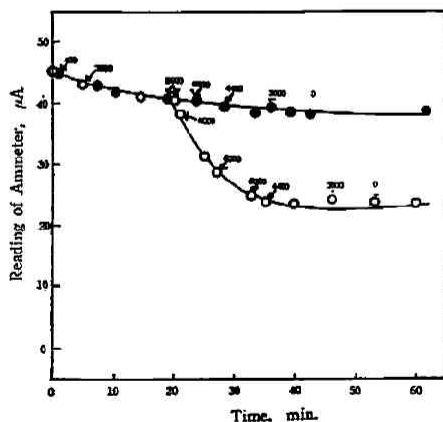
Fig. 8 Changes of light intensities passing through the pH 6.8 ovalbumin solutions (protein conc. 0.5%) on compressions —○—: Containing 1/40M phosphate buffer solution. —●—: Salt-free solution adjusted with 0.1N sodium hydroxide. Numerals in figure show pressure magnitude in the unit of \text{kg}/\text{cm}^2 .
