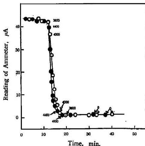
Fig. 7 Changes of light intensities passing through the pH 4.8 ovalbumin solutions (protein conc. 0.5%) on compressions —○—: Containing 0.1M acetate buffer solution. —●—: Salt-free solution adjusted with 0.1N hydrochloric acid. Numerals in figure show pressure magnitude in the unit of \text{kg}/\text{cm}^2 .
