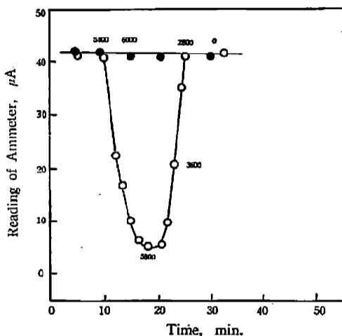
Fig. 11 Changes of light intensities passing through the pH 6.8 HSA solutions (protein conc. 0.5%) on compressions -○-: Containing 1/20M phosphate buffer solution. -●-: Salt-free solution adjusted with 0.1N sodium hydroxide.
