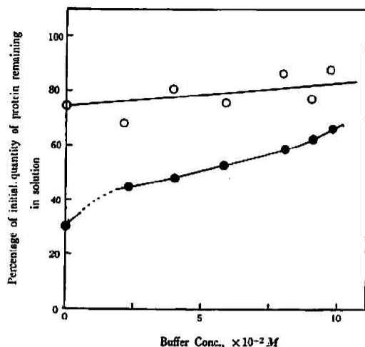
Fig. 12 The amounts of precipitation of HSA compressed at various buffer concentrations in sodium sulfate
