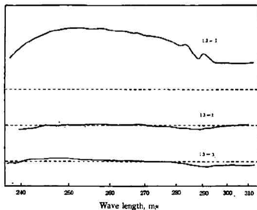
Fig. 13 Difference spectra of ultraviolet absorption of the compressed ovalbumin and HSA solutions in reference to their native solutions
