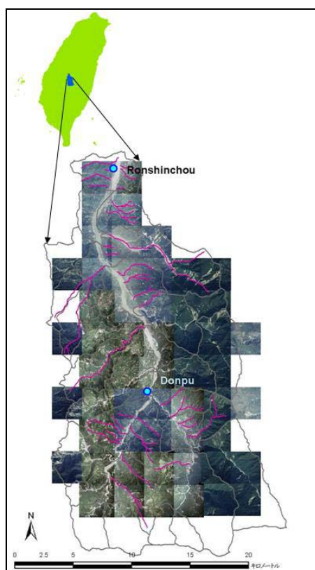
Fig.3 The Chenyoulunxi basin
