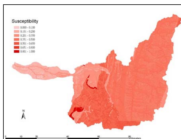
Fig.6 The result from discrimination analysis
