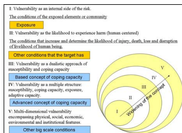
Fig.1 The concept of vulnerability (modified from Birkmann, 2007)
