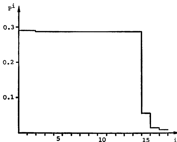
Fig. 5 The decreasing curve of p^i by the solution shown in Table 5.
