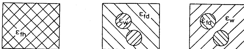
Fig. 13. Schematic presentation of the mixture model of CA matrix and water.
