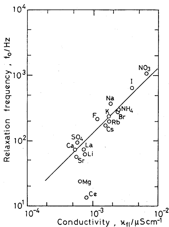
Fig. 10. Dependence of the relaxation frequency f_0 on the conductivity \kappa_H of the CA membrane immersed in different types of salt solutions of concentration 0.02 eq./l.
