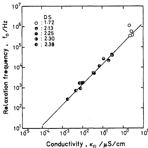
Fig. 7. Dependence of the relaxation frequency f_0 on the conductivity \kappa_{fl} of the CA membranes immersed in a 20 mM NaCl solution.
