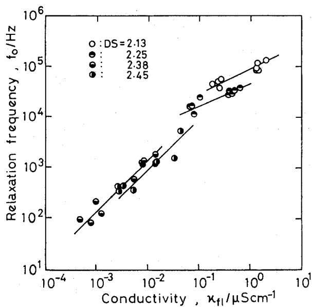
Fig. 9. Dependence of the relaxation frequency f_0 on the conductivity \kappa_H of the CA membranes immersed in NaCl solutions of different concentrations.
