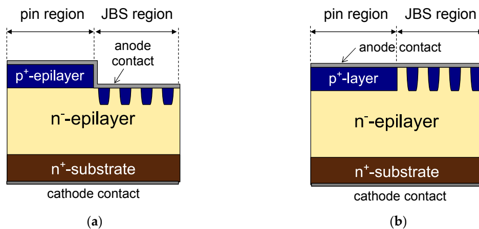
Figure 7. Schematic structures of SiC MPS diodes fabricated in this study. The main junction was formed by either (a) epitaxial growth or (b) \text{Al}^+ ion implantation. The widths of the pin and JBS (Junction-Barrier Schottky) regions were both 150 \mu\text{m} and of a stripe-like geometry. The active area was 3.6 \times 10^{-3} \text{ cm}^2 .
