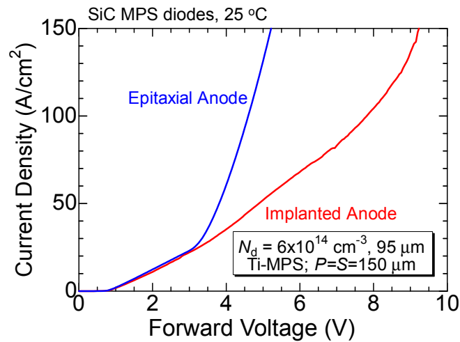
Figure 8. Forward characteristics for two types (epitaxial or implanted anode) of SiC MPS diodes fabricated in this study. The widths of the pin-region ( P ) and JBS region ( S ) were both 150 \mu\text{m} .
