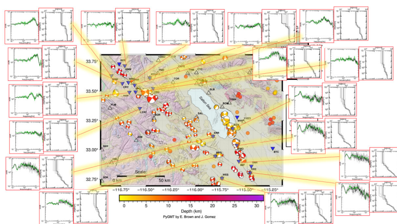
Fig.5 Locations of 17 SM sites locations in the Anza and Imperial Valley region where earthquake-HVSR spectra (left of subplots) are used to invert for V_S profiles (right of subplots).
