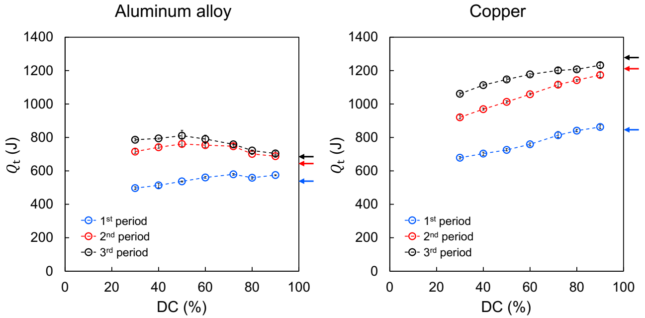
Fig. 12 Amounts of heat removed during each period: (left) aluminum alloy and (right) copper.
