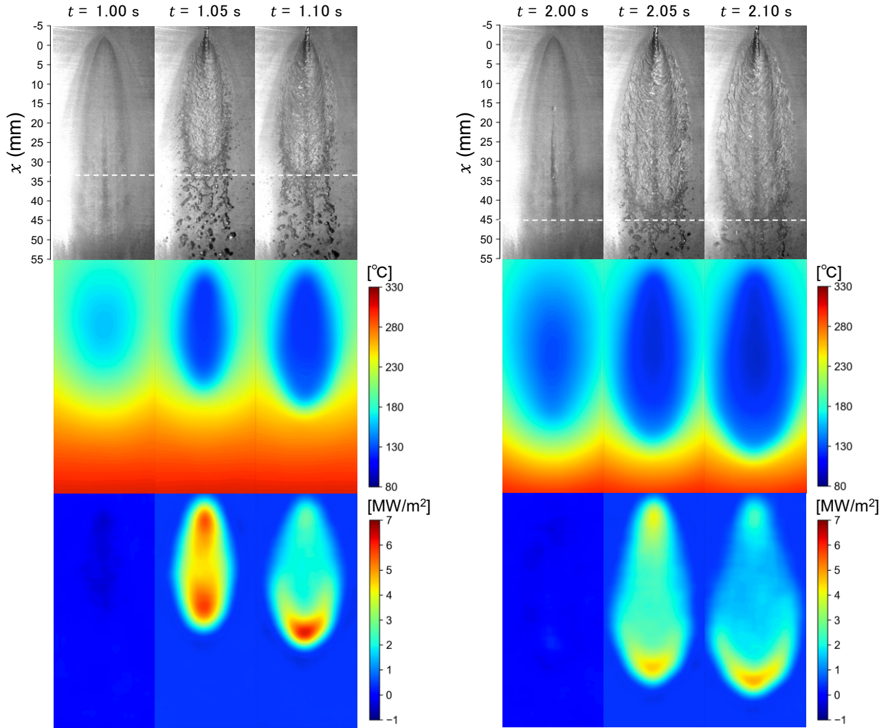
Fig. 6 Propagation of the liquid film during the 2 nd (left) and 3 rd (right) periods: images (upper), and estimated temperature (middle) and heat flux (bottom) distributions on the front surface. White dashed lines in each image indicate the wetting front position at the end of the previous ON time.
