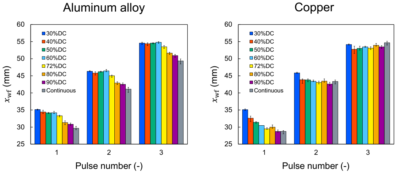
Fig. 8 Wetting front position at end of each ON time; (left) aluminum alloy, (right) copper.
