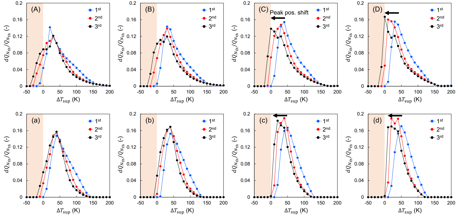
Fig. 14 Contribution of removed heat per degree of wall superheat to the total amount of heat removed during each period. (A, a) 30% DC, (B, b) 50% DC, (C, c) 80% DC, (D, d) continuous injection. Capital letters and small letters represent the results for the aluminum alloy and copper plates, respectively.
