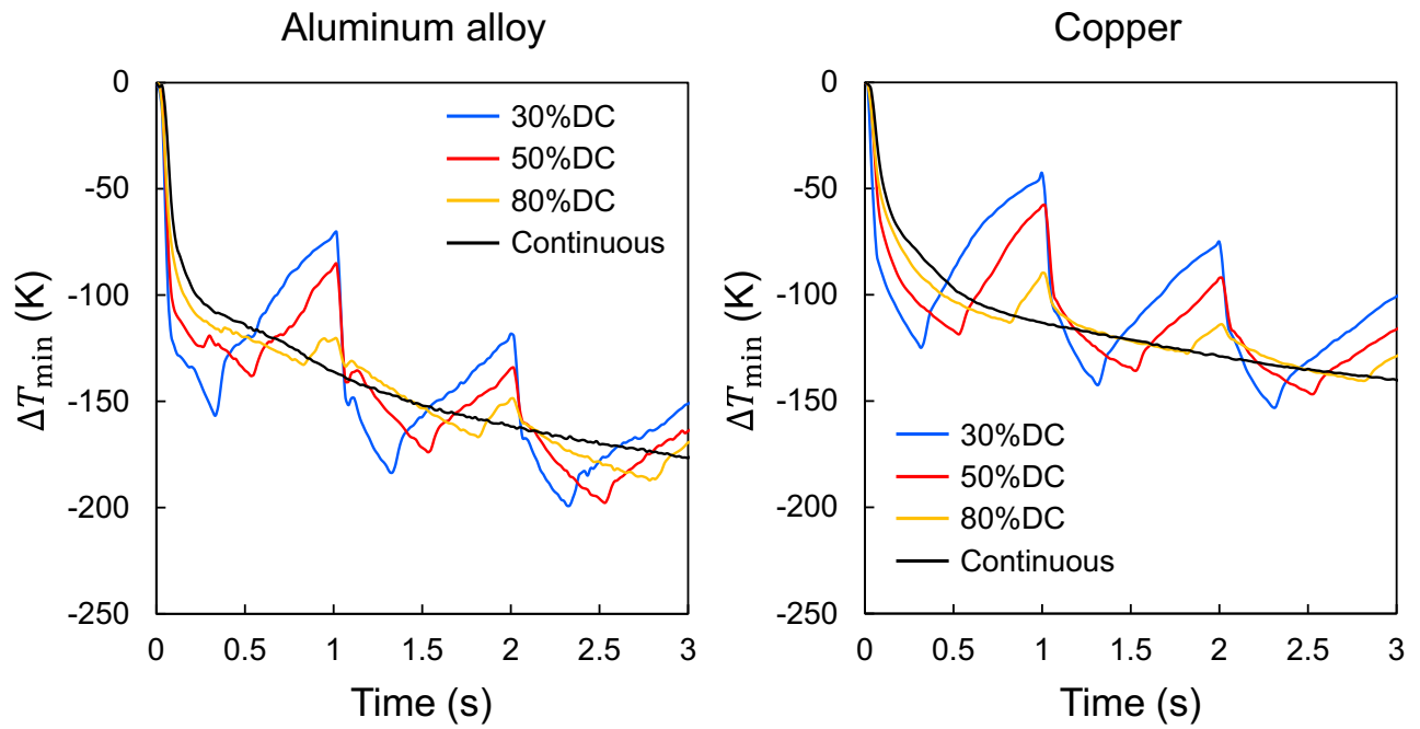
Fig. 13 Time histories of the minimum values of the temperature differences defined in Eq. (8): (left) aluminum alloy and (right) copper.
