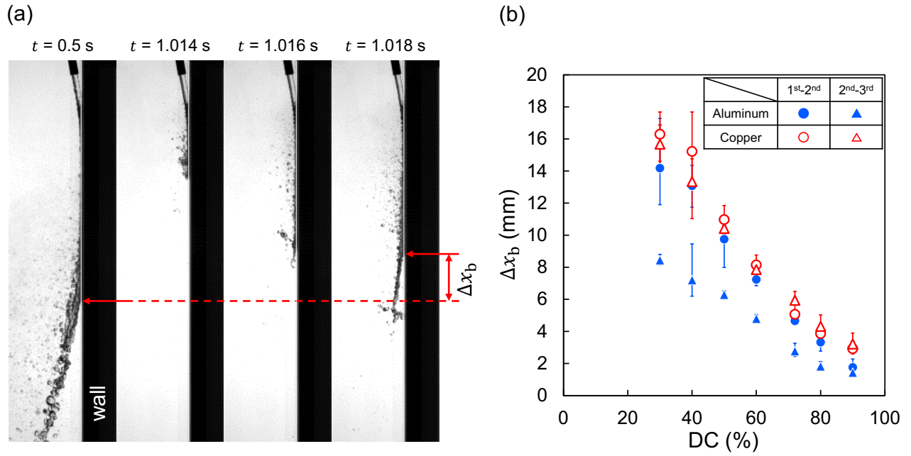
Fig. 9 (a) Side view of the propagation process of liquid films after re-injection, and (b) \Delta x_b values under each condition.
