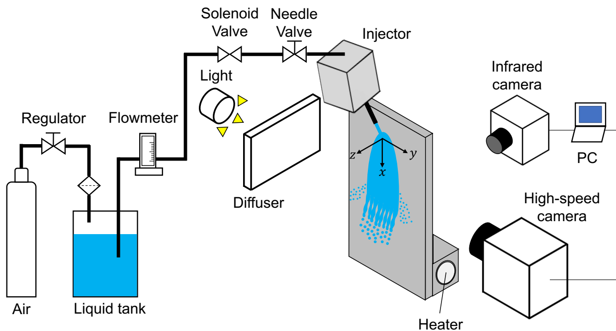
Fig. 2 Schematic of the experimental apparatus.
