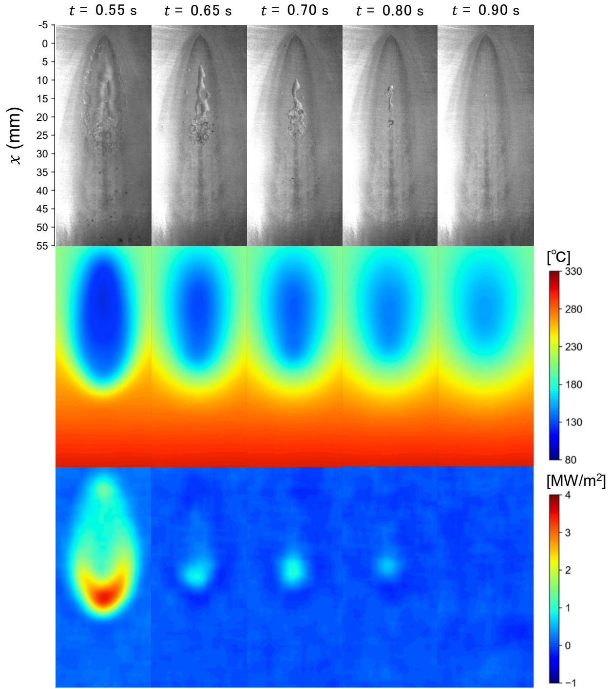
Fig. 5 Evaporation process of liquid film during the 1 st OFF time: images (upper), and estimated temperature (middle) and heat flux (bottom) distributions on the front surface.
