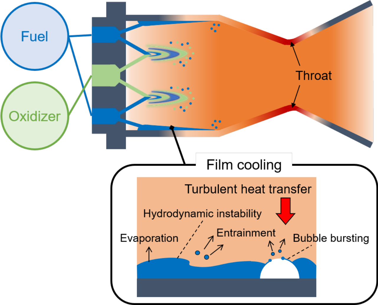
Fig. 1 Schematic of film cooling in the combustion chamber of bipropellant thrusters.
