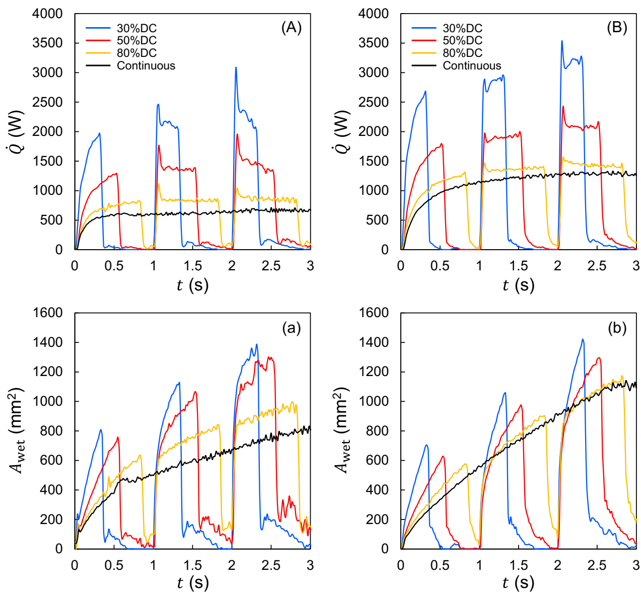
Fig. 11 Time histories of the rate of heat transfer and wetted area: (A, a) aluminum alloy and (B, b) copper.
