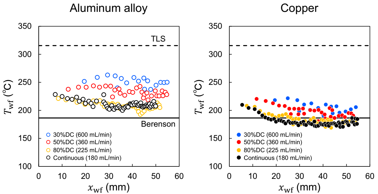
Fig. 10 Temperatures at the wetting front; (left) aluminum alloy, (right) copper.
