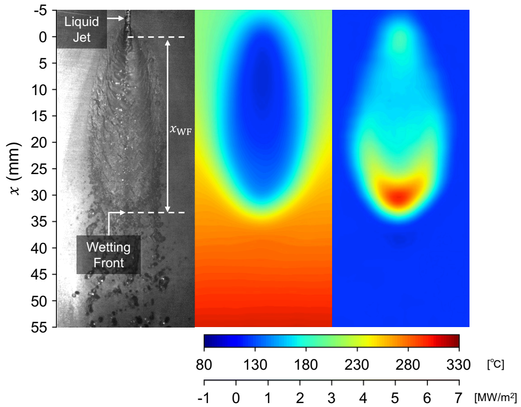
604 Fig. 4 Liquid film (left), and estimated temperature (middle) and heat flux (right) distribution on the 605 front surface at t = 0.5 s.
