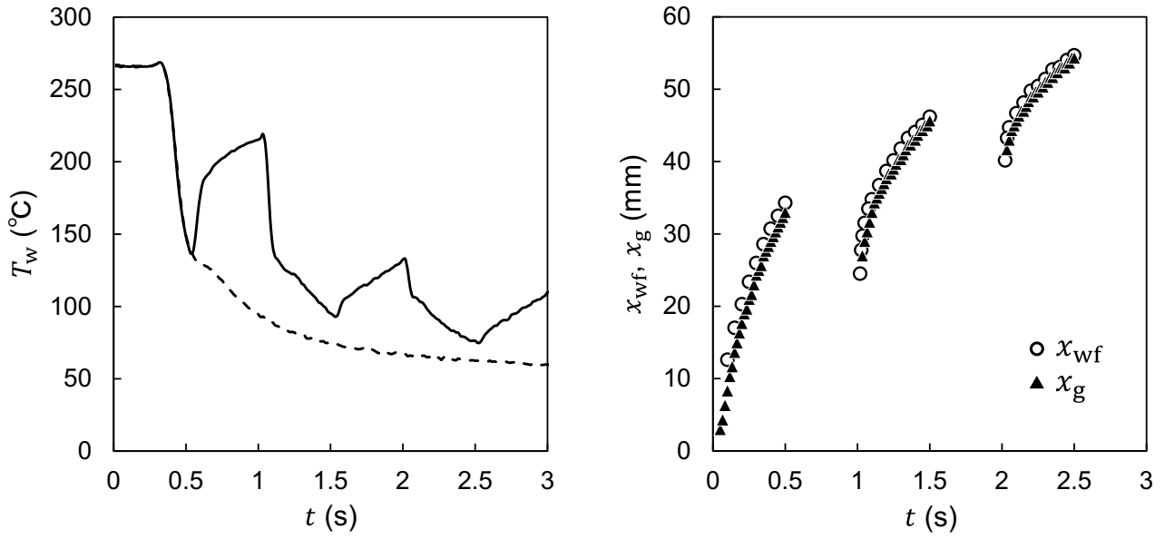
Fig. 7 Time histories of the temperature at x = 30.3 mm on the x axis and positions of x_{wf} and x_g .
