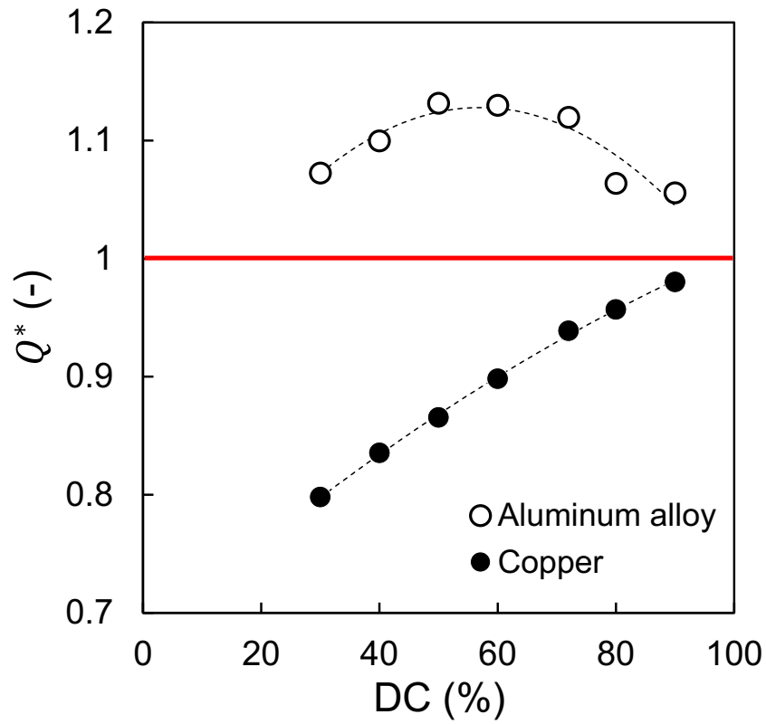
Fig. 15 Nondimensional heat removed by liquid film calculated using Eq. (9).
