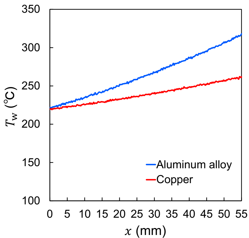
Fig. 3 Initial temperature distribution along the x axis.
