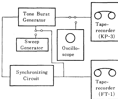
Fig. 2. Block diagram.
