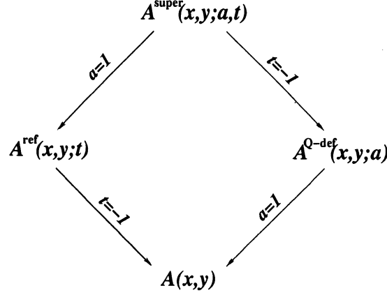
Fig 1: Hierarchy of A-polynomials
