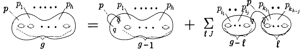
Fig. 2: Diagrammatic representation of the Eynard-Orantin's topological recursion relation (55)
