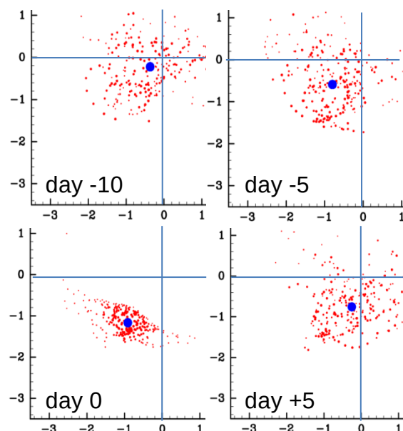
Fig. 6 Time evolution of the observed sample data residing in the vicinity of the point O : (PC1, PC2)=(-1.0, -1.4) at day 0 in the 2D phase space. Blue dots indicate their centroids.
