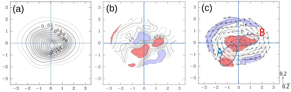
Fig. 3 (a) The observed PDF in 2D phase space spanned by the two-leading EOFs. The x - and y - axes correspond to PC1 and PC2, respectively. (b) Inhomogeneity of the observed PDF compared with multivariate Gaussianity. Percentages of random 10000 PDFs having smaller values than the observation are shown by contours. Regions larger (smaller) than 80 (20) % are shaded with warm (cool) color. The additional dotted contours are 95% and 5%. (c) Averaged phase-space velocity vectors \mathbf{V} (arrows) in the 2D phase space. Contours show the magnitude of the vector |\mathbf{V}| . Regions where |\mathbf{V}| > 0.16/\text{day} ( < 0.08/\text{day} ) are shaded by cool (warm) color. Regions corresponding to regimes A and B are shown by colored ellipsoids.
