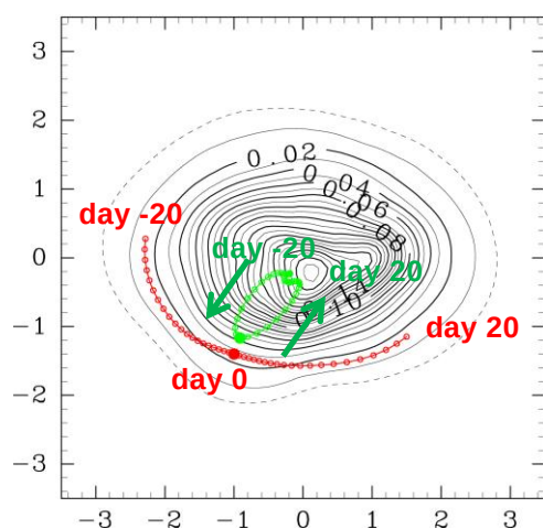
Fig. 5 Trajectory passing through the point O : (PC1, PC2)=(-1.0, -1.4) representing regime A. Small dots indicate daily position. The red curve shows the trajectory estimated by the averaged phase-space velocity in Fig. 3c, while the green curve is obtained from centroids of the observed sample data residing in the vicinity of the point O at day 0.
