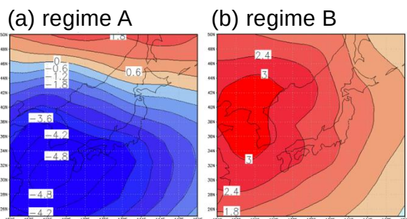
Fig. 4 Horizontal distribution of 850-hPa temperature anomaly for the representative points of (a) regime A: (PC1, PC2)=(-1.0, -1.4) , and (b) regime B: (PC1, PC2)=(1.0, 0.0) .
