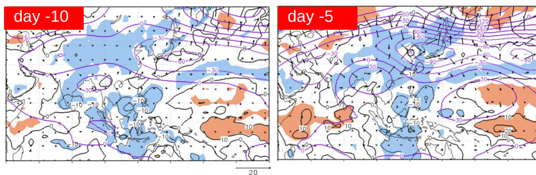
Fig. 8 As in Fig. 7 except for the anomaly of OLR (black contour; \text{W/m}^2 ) and 250-hPa stream-function ( \times 10^5 \text{ m} ). Regions with a statistical significance over 99% for OLR anomaly are color shaded.
