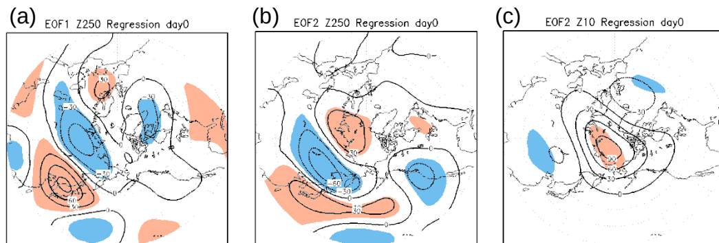
Fig. 2 Simultaneous regressed map of 250-hPa geopotential height anomaly with respect to (a) PC1 and (b) PC2. (c) The regressed map of 10-hPa height anomaly with respect to PC2. Contour interval is 30 m. Regions with a statistical significance over 99% are color shaded.
