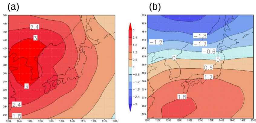
Fig. 1 Spatial patterns of (a) EOF1 and (b) EOF2 for low-frequency 850-hPa temperature variation over the Far East.
