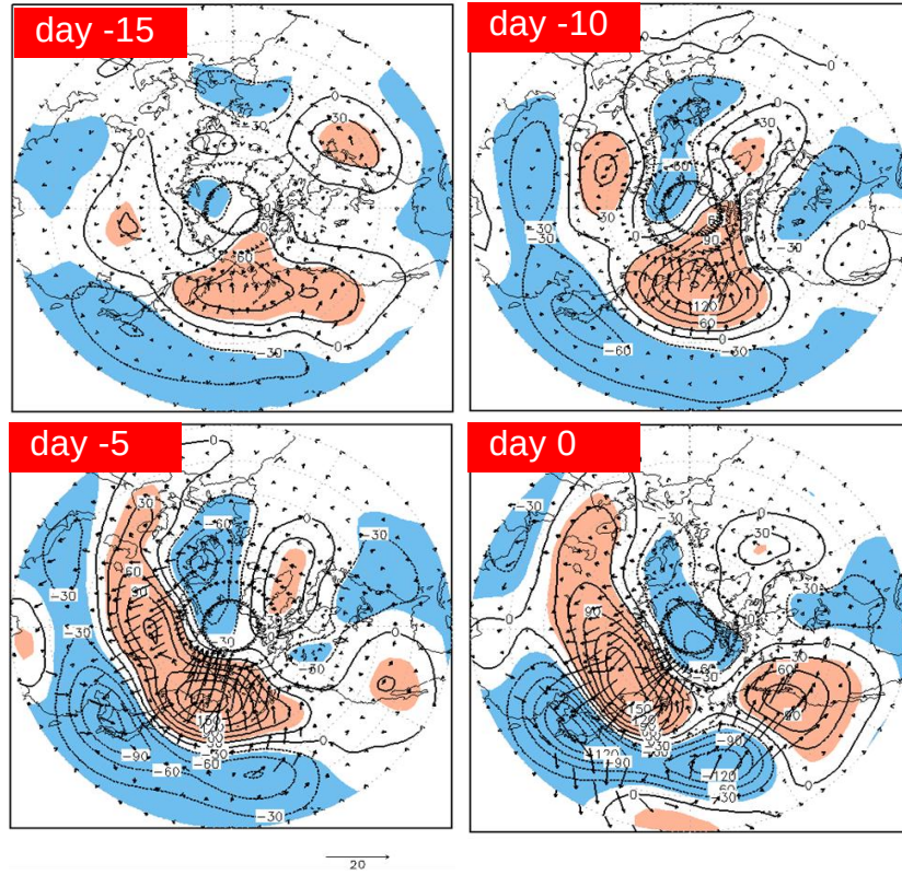
Fig. 7 Composited anomaly of 250-hPa geopotential height anomaly (m) corresponding to green dots in Fig.5. Contour interval is 30m, and regions with a statistical significance over 99% are color shaded. The arrows indicate wave-activity flux ( \text{m}^2/\text{s} ) of Takaya and Nakamura (1997).
