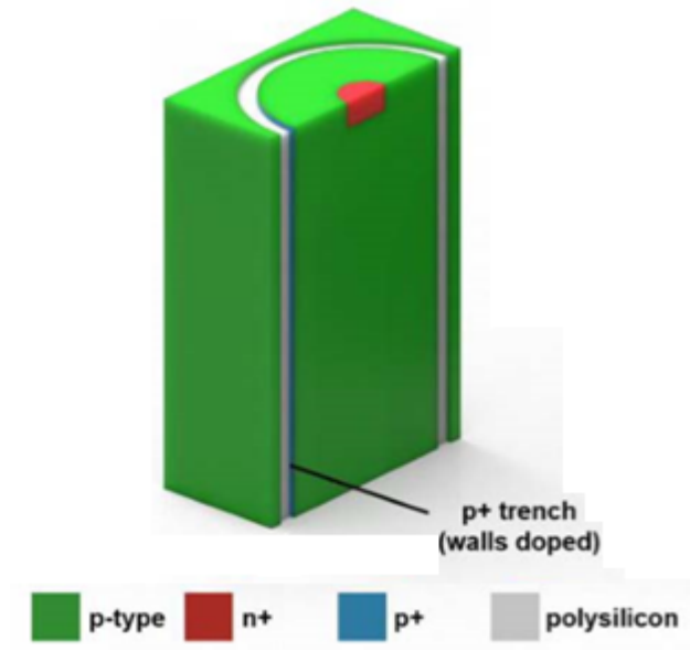
Figure 5.3: 3D schematic of the 3D mushroom microdosimeter.
