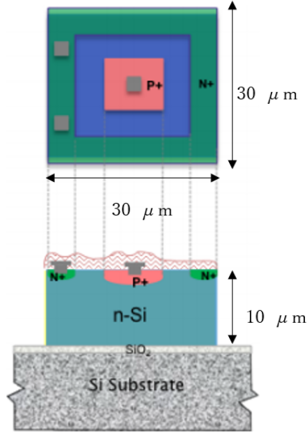
Figure 2.6: Schematic of the 3D bridge microdosimeter. Each sensitive volume is 30\text{ }\mu\text{m}\times30\text{ }\mu\text{m}\times10\text{ }\mu\text{m} (width \times length \times height). Image from [7].
