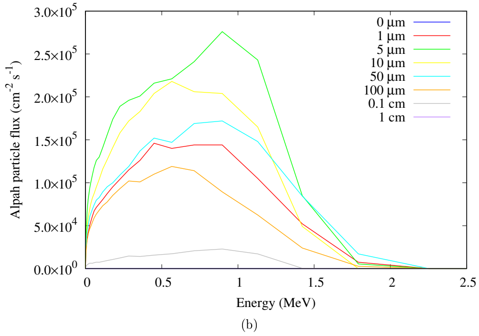
Figure 4.15: The alpha particle flux calculated inside the sensitive volume of the detector at various thickness of B4C converter for (a) KUR mix mode and (b) KUR epithermal mode.
