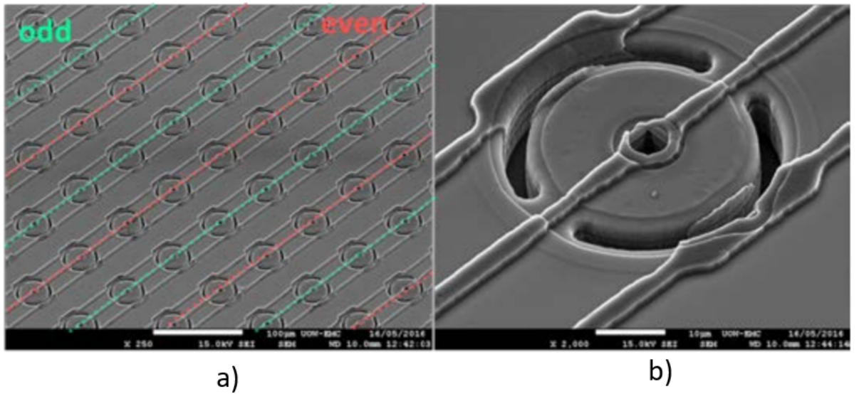
Figure 5.4: Scanning electron microgram image of 3D mushroom microdosimeter a) Array of sensitive volume showing the odd and even rows. b) Single sensitive volume.
