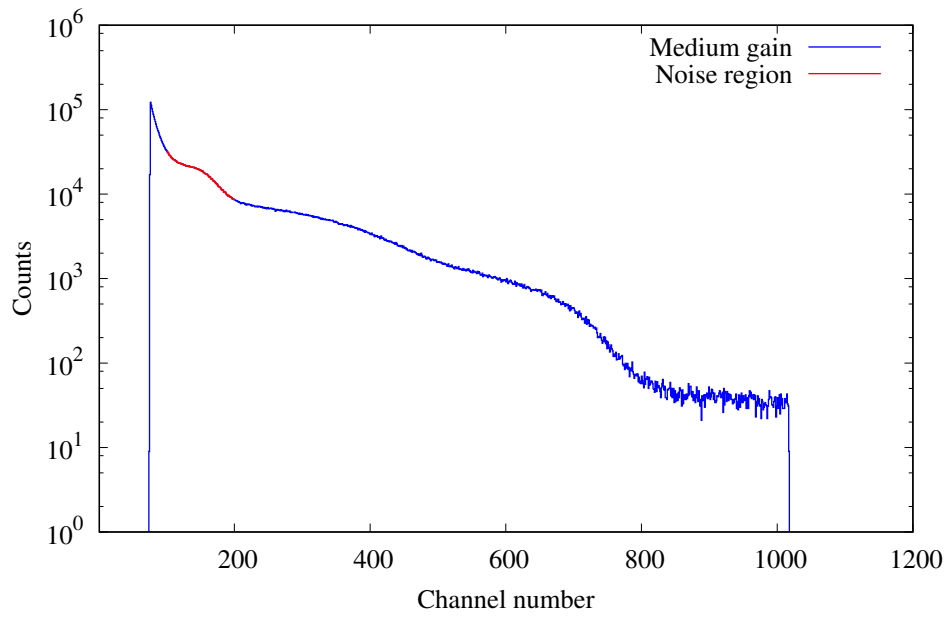
Figure 3.27: Raw spectrum of the epithermal neutron beam at KUR obtained with the TEPC. The red region indicates some static noise present in the electronic circuit.
