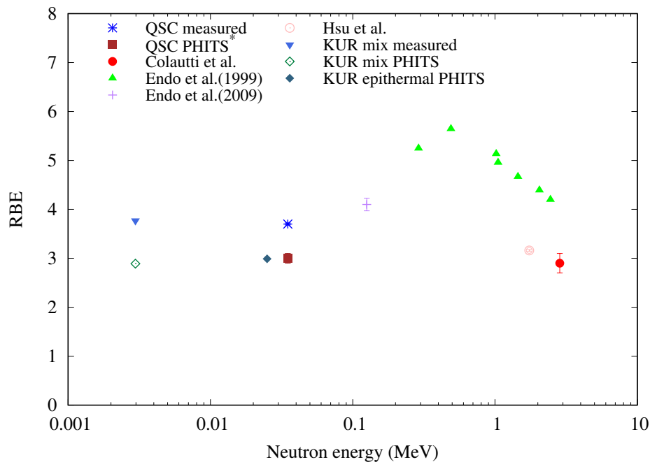
Figure 3.51: Comparison of RBE as a function of neutron energy calculated using a weighted biological function for various neutron sources.
