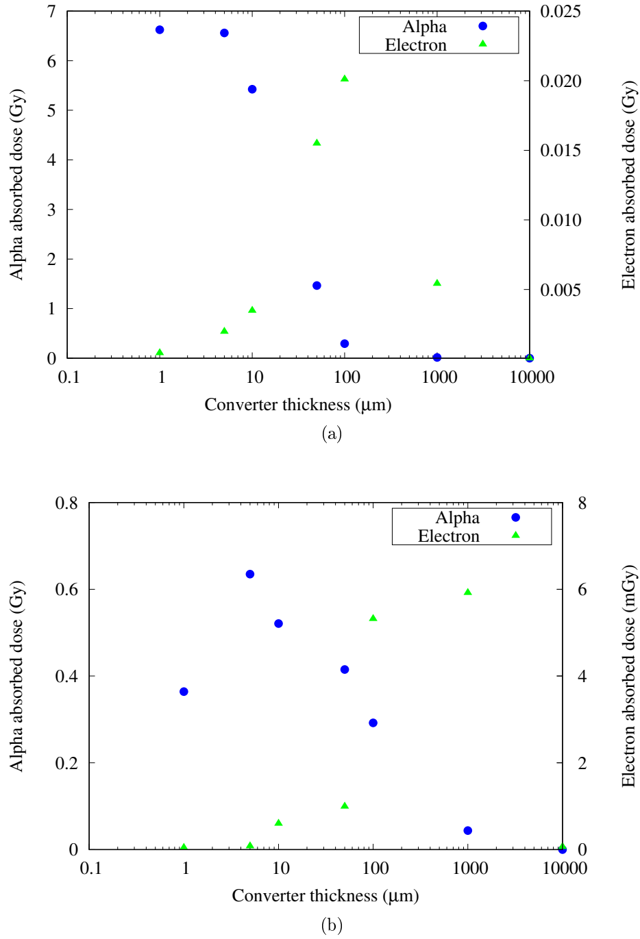
Figure 4.16: Alpha and electron absorbed dose calculated inside the sensitive volume at various converter thickness for (a) KUR mix mode and (b) KUR epithermal mode.
