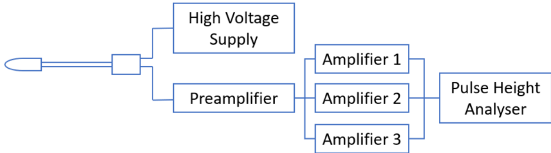
Figure 3.6: Electrical interconnection diagram for LET-1/2 operation.
