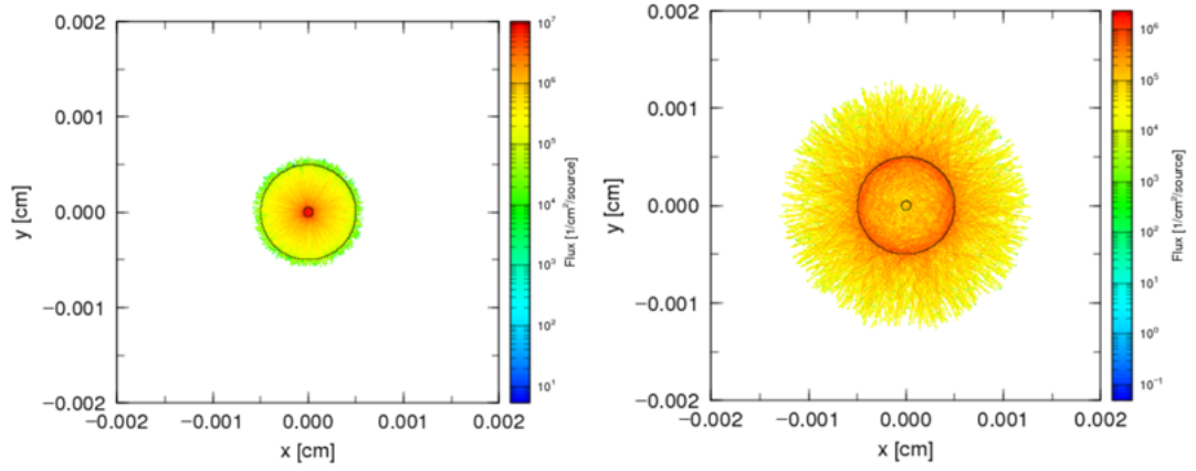
Figure 5.11: Ion track of 1.47 MeV alpha particles inside a single sensitive volume. Left) p+ core through the centre of the sensitive volume. Right) p+ ring on the outside of sensitive volume.
