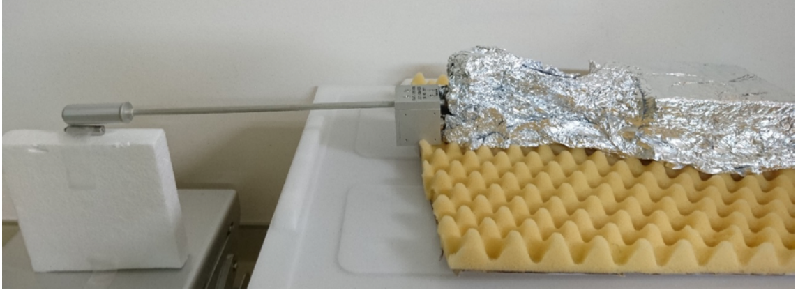
Figure 3.7: Image of the ^{252}\text{Cf} spectrum measurement using LET-1/2 detector.
