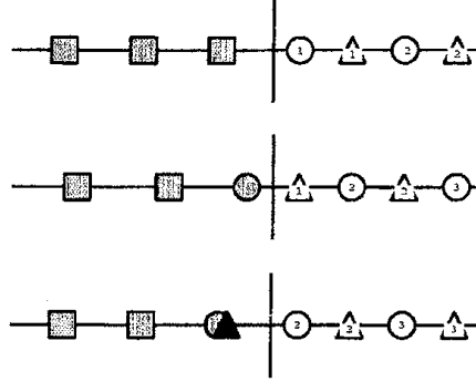
Figure 6: The formation of pairs. The square boxes on the negative real axis represent zeros of Stokes multipliers. The circles (triangles) represent energy levels with positive (negative) parity. Just distinguish them we assign number labels. The case \alpha < 3 (top), 3 < \alpha < 5 (middle), \alpha = 5^+ (bottom).
