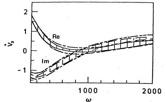
Fig. 2 The frequency characteristics of the voltage V_3 .
