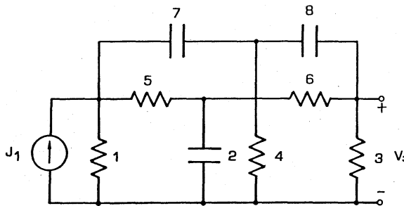
Fig. 1 Notch filter circuit.
