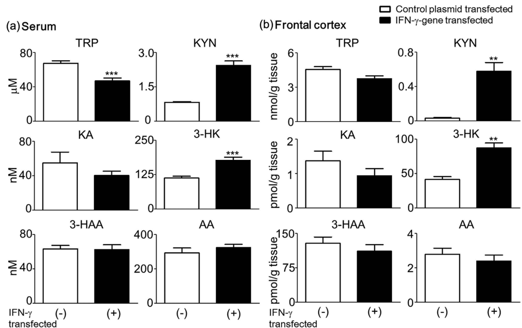
Figure 3. Changes in the levels of TRP and its metabolites in the serum and frontal cortex of mice after IFN- \gamma gene transfer. TRP-KYN metabolite concentrations were determined in the serum (a) and the frontal cortex (b) of mice at 28 days after IFN- \gamma -gene transfer. The open bar shows IFN- \gamma -transfected (-) mice, and the closed bar shows IFN- \gamma -transfected (+) mice. Each column represents the mean \pm SEM (n = 15–20). ** p < 0.01, *** p < 0.001 versus IFN- \gamma -transfected (-) mice.
