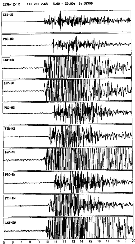
Fig. 4. Typical 3-component seismogram of Guntur volcanic earthquake recorded at four permanent stations.
