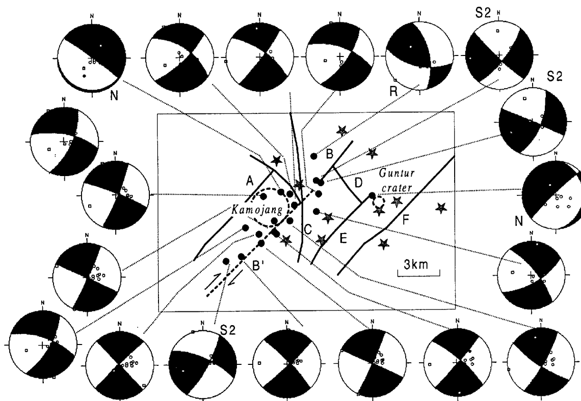
Fig.7. Source mechanisms of volcanic earthquake around Kamojang Caldera. Solid circles and stars represent epicenters and stations, respectively. Solid line indicate geological fault (Alzwar et al. , 1992) as shown by A-F. Focal mechanism diagrams are equal-area projection of the upper-hemisphere of the focal sphere.
