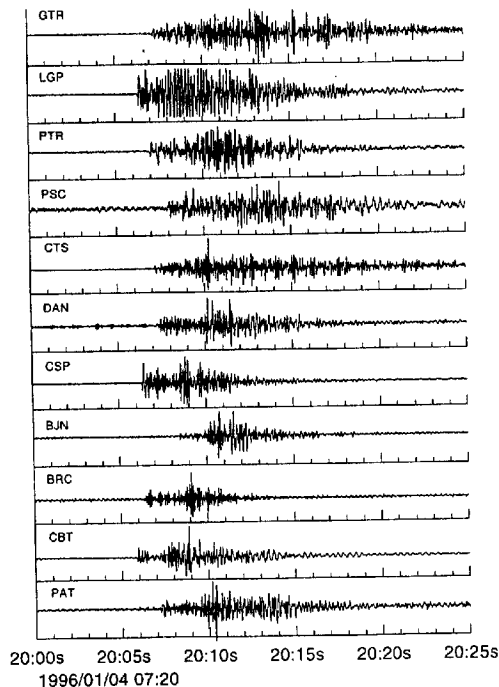
Fig. 5. An example of vertical component seismogram of Guntur volcanic earthquake recorded at temporary seismic stations.
