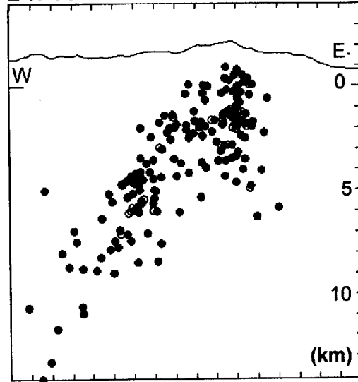
Fig.6 Hypocenter distribution around Guntur volcano in November 1994 – December 1996. Upper: epicenter, Lower: vertical cross-section of east-west direction. Crosses indicate stations.
