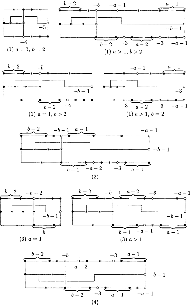
Figure 4: The dual graph of D + E_1 + E_2
