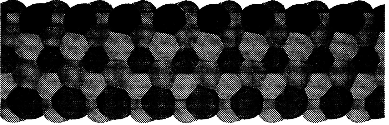
Figure 3: Ford domain of a quasifuchsian punctured torus group
