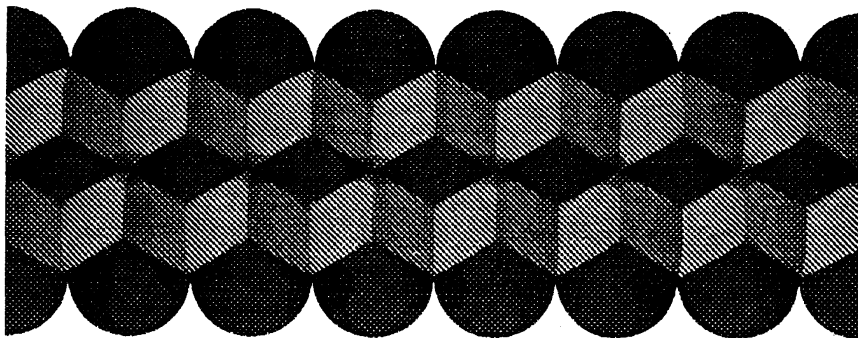
Figure 5: Ford domain for \sigma_0
