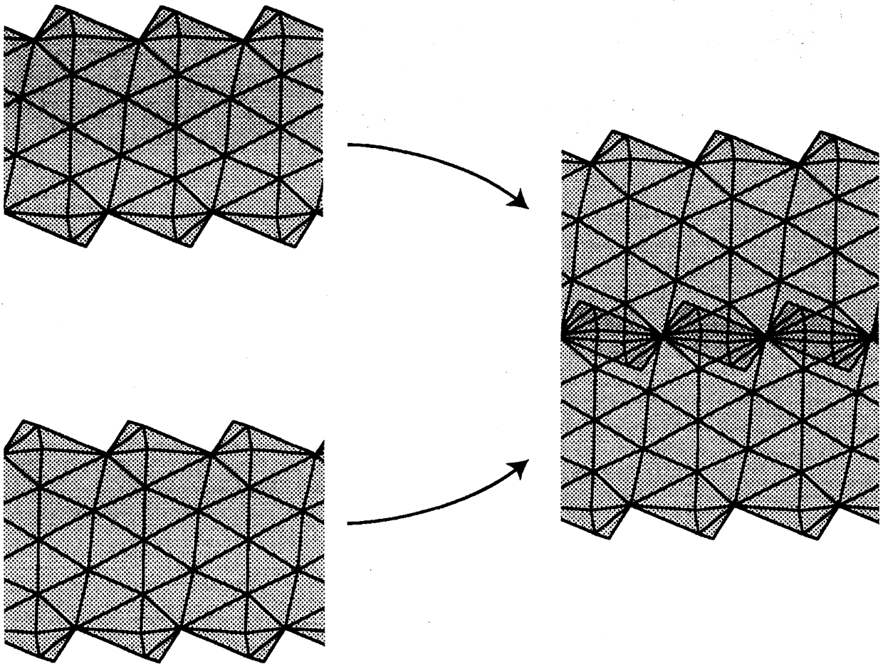
Figure 10: Idea of construction of the dual complex (1): The dual complex is based on two copies of the dual complex for a quasifuchsian punctured torus group
