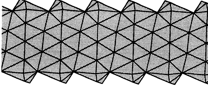
Figure 4: Dual of Ford domain
