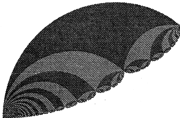
Figure 12: Conjectural picture of \mathcal{J}_{\text{sym}} for (p, q) = (3, 5)
