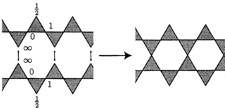
Figure 7: The link of the ideal vertex of \Delta_0^{1/2}
