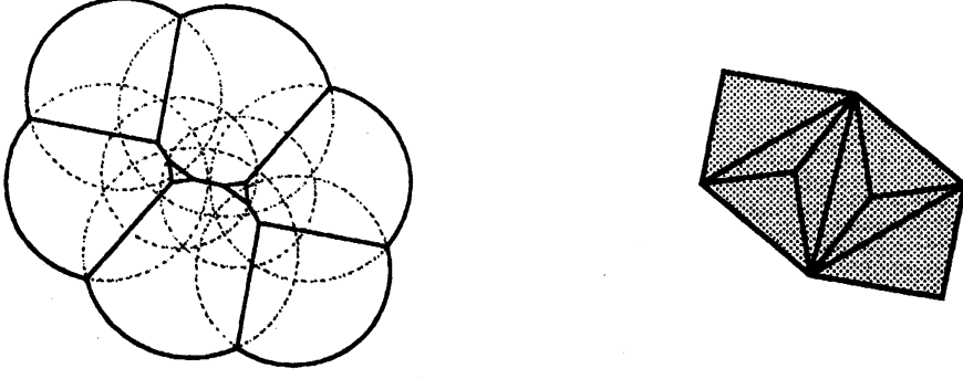
Figure 2: Ford domain of a cyclic Kleinian group and its dual
