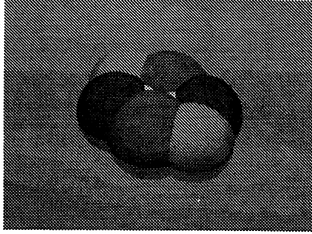
Figure 1: Ford domain of a cyclic Kleinian group
