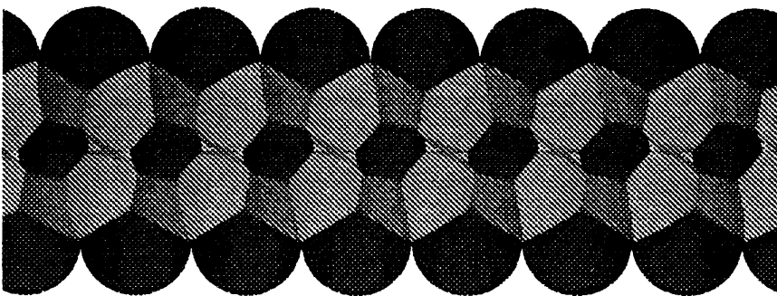
Figure 6: Ford domain for \sigma(3, 5)
