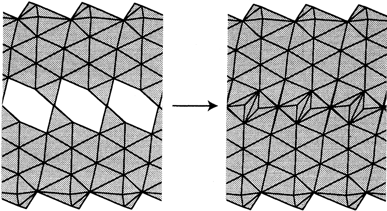
Figure 11: Idea of construction of the dual complex (2): By drilling and filling with the dual complex for a cyclic Kleinian group, we obtain the desired complex
