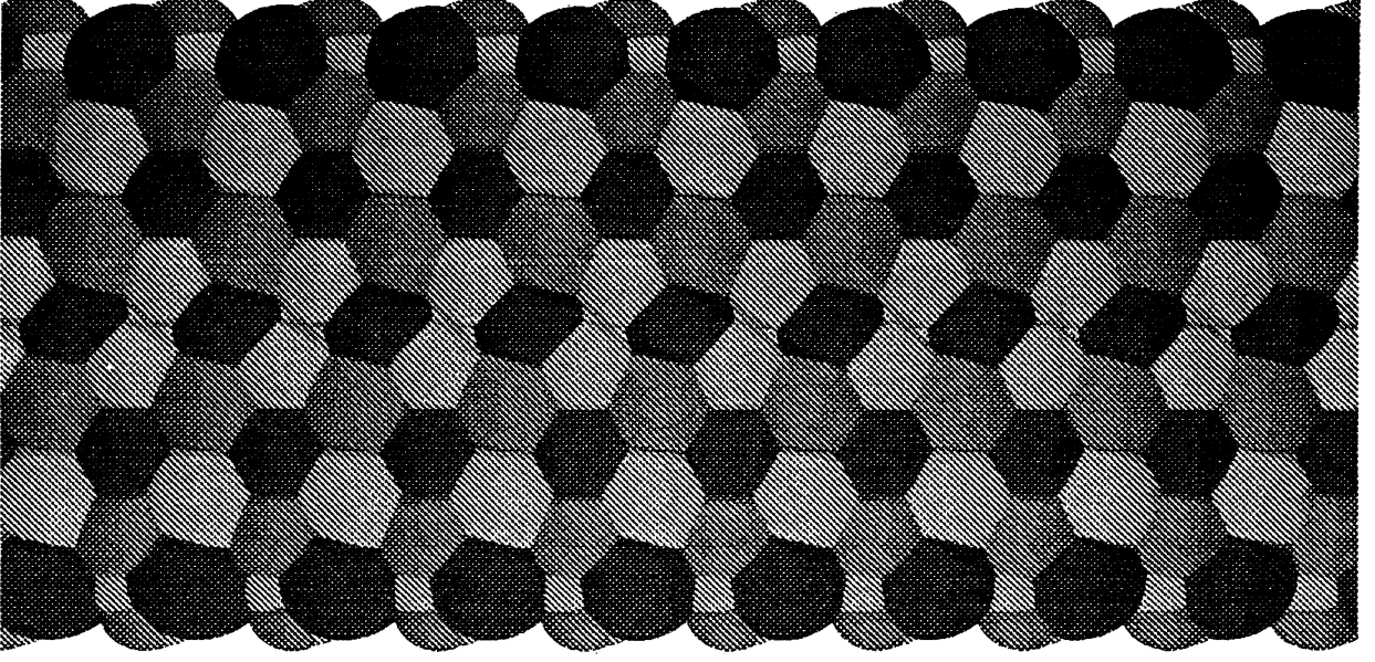
Figure 9: Ford domain for a hyperbolic structure in \mathcal{J}_{\text{sym}}^{\text{thick}} \subset \mathcal{MP}_{\text{sym}}(p, q) for (p, q) = (3, 5)
