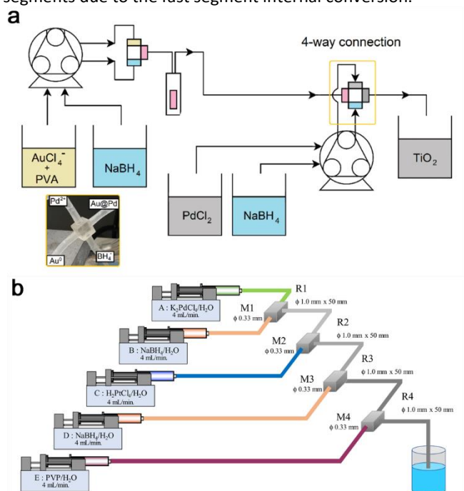
Fig. 4 Schematics of multi-step flow reactors for a) Au@Pd (the inset is the 3D printed 4-way connection) and b) Pd@Pt core-shell NPs. Reproduced with permission from ref. 40 Copyright 2019, Royal Society of Chemistry; ref. 41 Copyright 2021, Elsevier.
