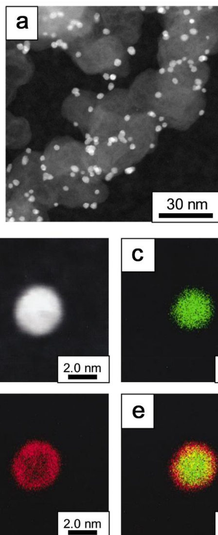
Fig. 5 (a) DF-STEM image of Pd@Pt. (b) DF-STEM image and its EDS maps of (c) Pd and (d) Pt and (e) Pd + Pt. Reproduced with permission from ref. 41 Copyright 2021, Elsevier.
