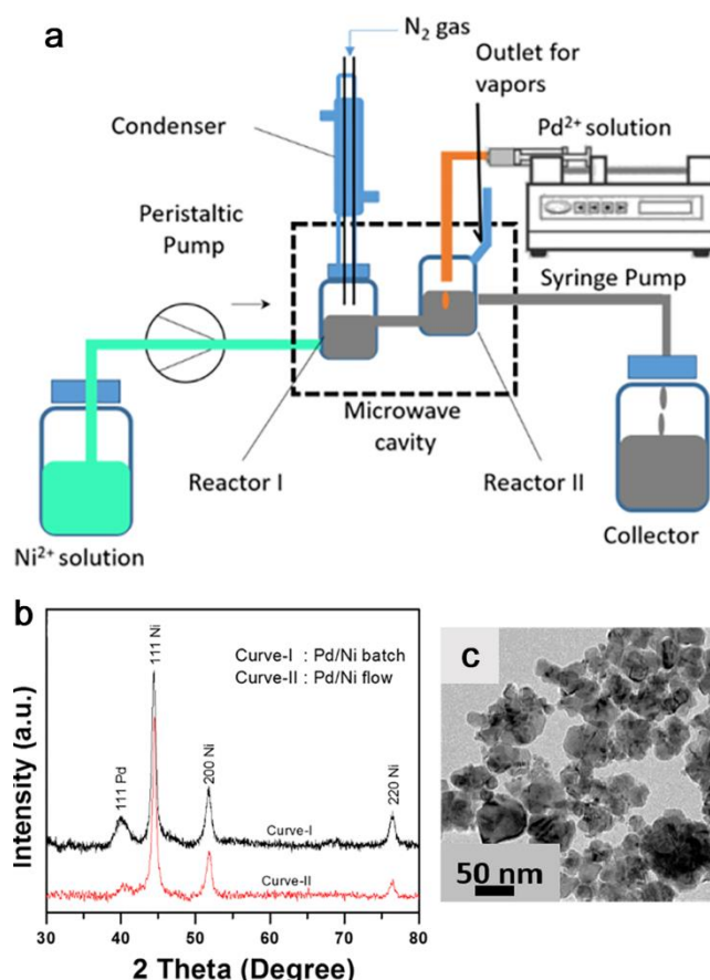
Fig. 7 (a) Schematic of microwave-assisted continuous-flow reactor for the sequential reduction of Ni and Pd ions. (b) Powder XRD patterns of Pd/Ni samples synthesized by batch (Curve-I) and flow (Curve-II) methods. (c) TEM image of Pd/Ni samples synthesized by the flow method. Reproduced with permission from ref. 50 Copyright 2017, American Chemical Society.
