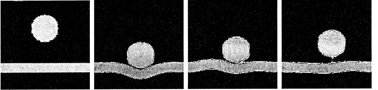
Figure 3: Example of elastic-plastic flow. The system is described by 100 \times 100 Cartesian fixed grid and only 10 grids are used for the width of plate. Plate and ball are moving through fixed grid system. Black part is filled with air and is also calculated.
