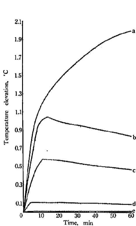
Fig. 4 Temperature and time relations for the reactions between enzyme U_8 and urea of various concentrations in the presence of buffer pH=6.70
