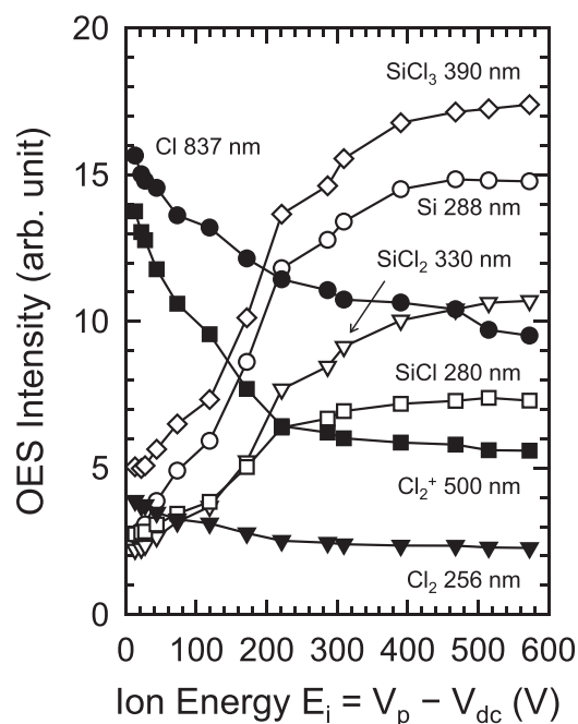
FIG. 12. OES intensities of seven species \text{SiCl}_x ( x=0-3 ), \text{Cl}_x ( x=1, 2 ), and \text{Cl}_2^+ as a function of ion incident energy in the range E_i \approx 13-570 eV, measured during ICP plasma etching of Si in \text{Cl}_2 under the same conditions as in Fig. 2. The wavelengths and transitions for the atomic and molecular emissions concerned are listed in Table I.
