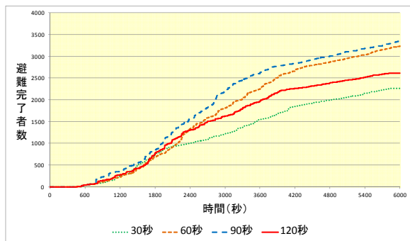
Fig. 8 The number of pedestrians who complete evacuating under various signal durations
