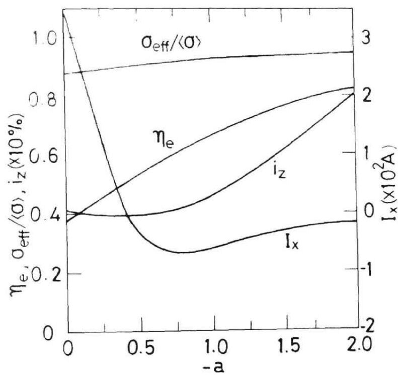
Fig. 2.67. Influence of a on I_x , i_z , \eta_e , and \sigma_{\text{eff}}/\langle\sigma\rangle when \kappa \doteq 0.5 and T_w = 1600 \text{ K} .
