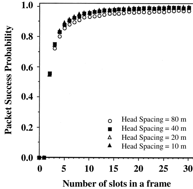
Fig. 5.7 Success probability of a reply packet.
