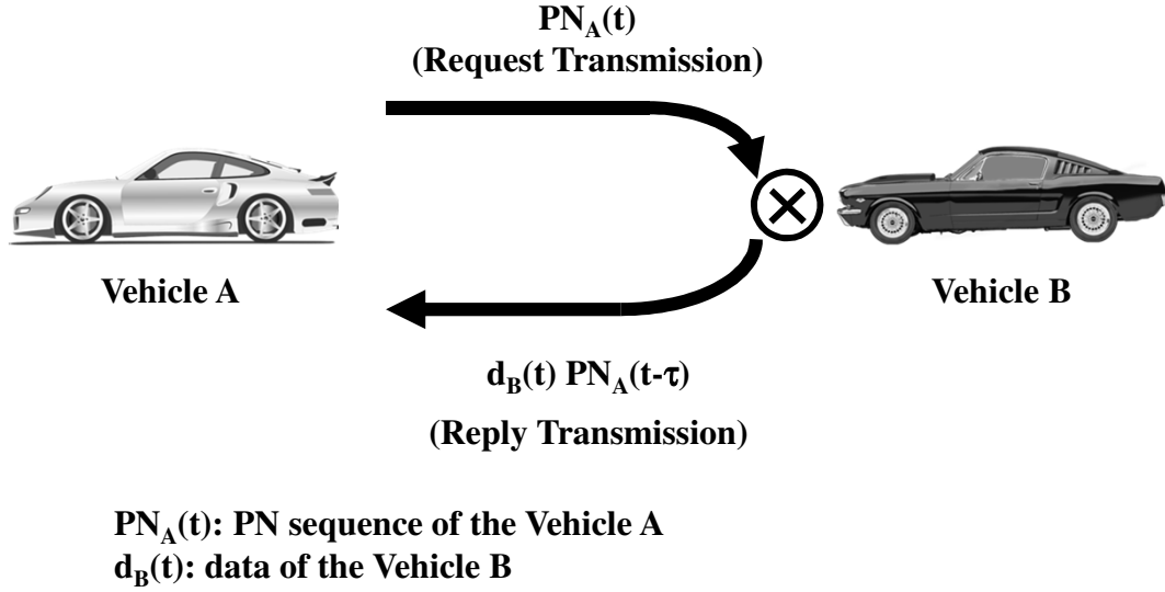
Fig. 5.2 Principle of Spread Spectrum Boomerang Communication.
