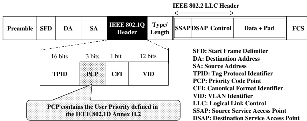
Fig. 3.1 User priority information contained in an Ethernet frame.
