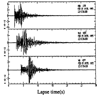
Fig. 3. Examples of waveforms of the vertical component for the analysis of Q_c . The waveforms of ABU, MYO and YGI stations are shown. Lapse time is measured from the origin time.
