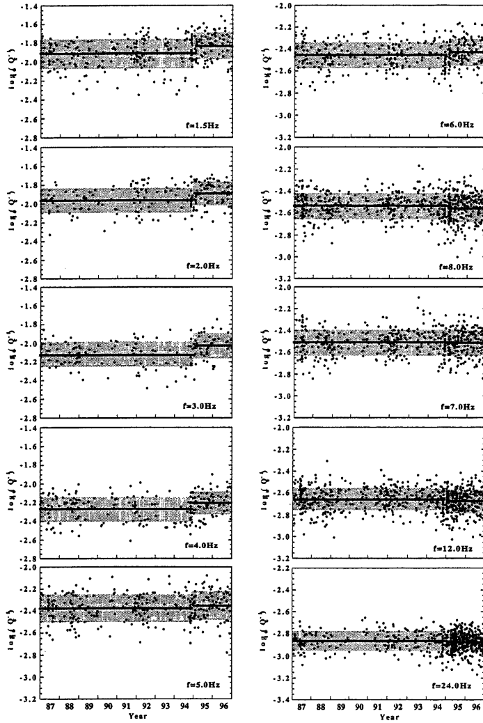
Fig. 9. The temporal variation in Qc^{-1} bounded by the occurrence of the Hyogo-ken Nanbu earthquake. Solid lines show the average and hatched zones the standard deviation of each time window. At lower frequency bands the average of Qc^{-1} increases after the earthquake.
