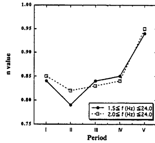
Fig. 12. The temporal variation in the power of frequency n for Q_c^{-1} . Solid circles show the n values which are determined by all the data of from 1.5 to 24 Hz. Open squares show the n values which are determined by the data of from 2.0 to 24 Hz to reduce the fluctuation of Q_c^{-1} at low frequency due to surface wave.
