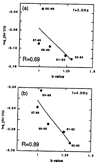
Fig. 13. The correlation between b value and Q_c^{-1} at (a) 3.0 Hz and (b) 4.0 Hz. Both figures show a negative correlation between Q_c^{-1} and b value.
