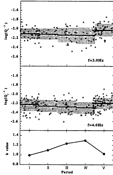
Fig. 11. The comparison of the temporal variation of Q_c^{-1} at frequency bands of (a) 3.0 and (b) 4.0 Hz with that of (c) b value. Q_c^{-1} decrease from I to IV and increases IV to V at both frequency bands. The b value increase from I to IV and decreases from IV to V. Note that the temporal variation in Q_c^{-1} is reverse to that of b value.
