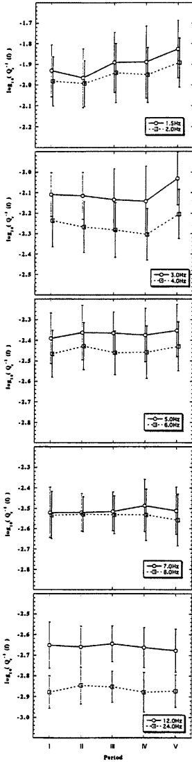
Fig. 10. The temporal variation in Q_c^{-1} for five periods (I-V) of two years. Q_c^{-1} at the frequency bands of 3.0 and 4.0 Hz increases significantly from IV to V, corresponding to the occurrence of the Hyogo-ken Nanbu earthquake.
