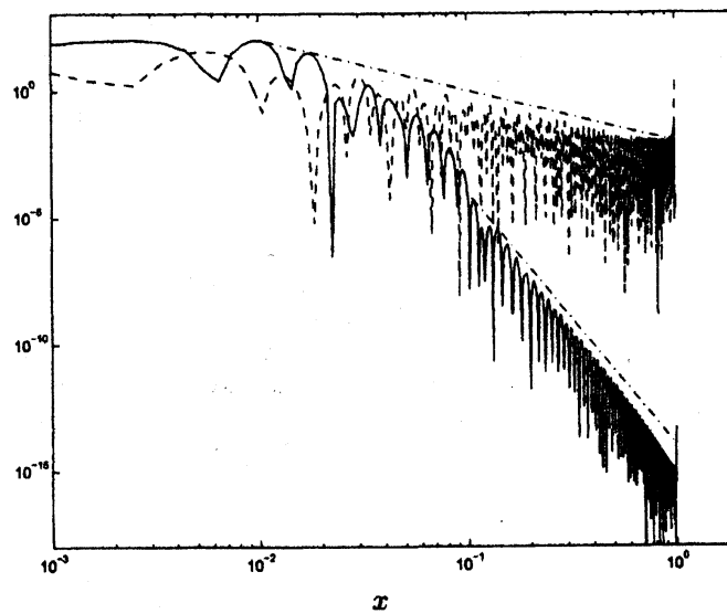
Figure 2: Decay of the square of the wavelet functions \psi_{ji}^2(x) with scale index j = 8 and position index i = 128 . The lower curve corresponds to the present basis, the upper one to the basis of Fröhlich and Uhlmann (2002). The straight reference lines are proportional to x^{-10} and x^{-2} , respectively.
