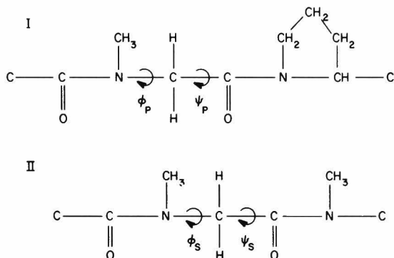
Fig. 7. Element dipeptides, Sar-Pro (I) and Sar-Sar (II).
