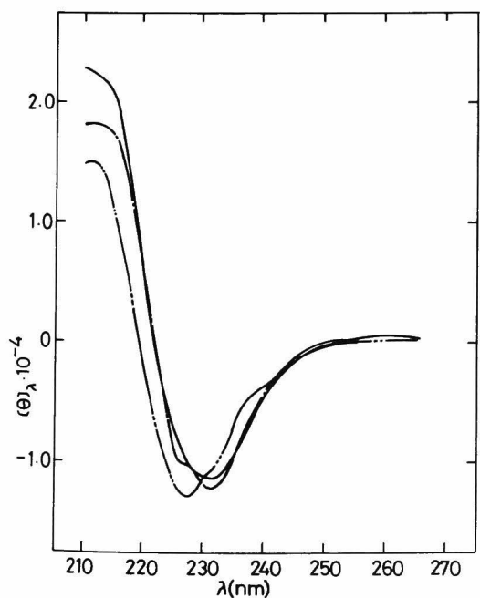
Fig. 7. Change of cd spectrum of c(\text{PSS})_2 in dioxane/ethanol (4/5 v/v) mixed solvent induced by DL-p-MeOPhe-OEt·HCl. Molar ratio of (DL-p-MeOPhe-OEt·HCl)/( c(\text{PSS})_2 ): —, 0; - - -, 3.0; - · - ·, 6.0.
