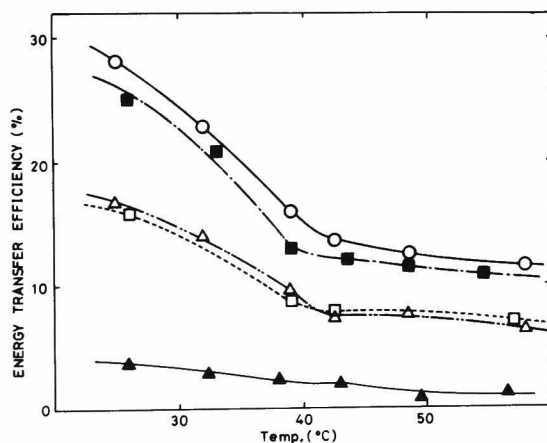
Fig. 5. Temperature dependence of the energy-transfer efficiency under various probe concentrations. (Boc-Try-Phe-OEt)/(12-AS): ○, 3.3 \times 10^{-6} M/ 3.3 \times 10^{-6} M; ■, 1.65 \times 10^{-6} M/ 3.3 \times 10^{-6} M; □, 3.3 \times 10^{-6} M/ 1.65 \times 10^{-6} M; △, 1.65 \times 10^{-6} M/ 1.65 \times 10^{-6} M; ▲, 3.3 \times 10^{-7} M/ 3.3 \times 10^{-7} M.
