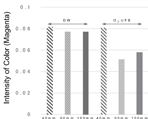
Fig. 7 Confirmation of the cleaning effect of standard contaminated sheets (Color intensity Normalized with Magenta).
