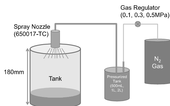
Fig. 1 Experimental Facility.
