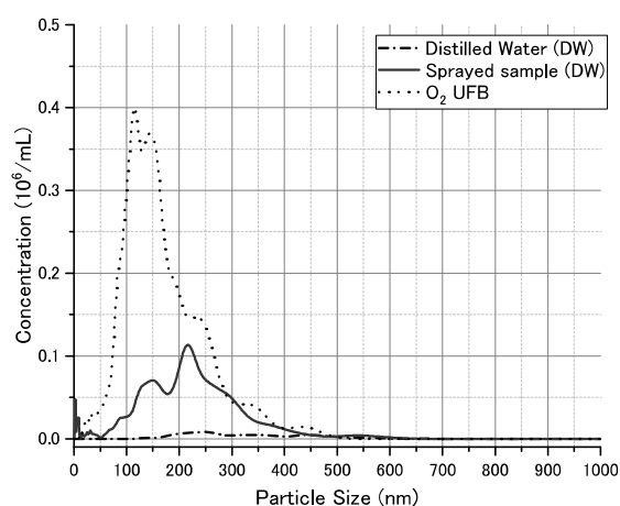
Fig. 2 UFB distribution before and after droplet.
