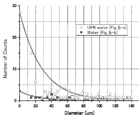
Fig. 6 Micro bubble distribution by high-speed camera analysis.
