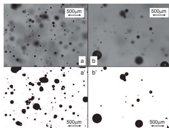
Fig. 5 High-speed image of ejected water with/without O 2 UFB (a: original photo of ejected water with UFB; b: original photo of ejected water without UFB; a': photo a after analyze particles; b': photo b after analyze particles).
