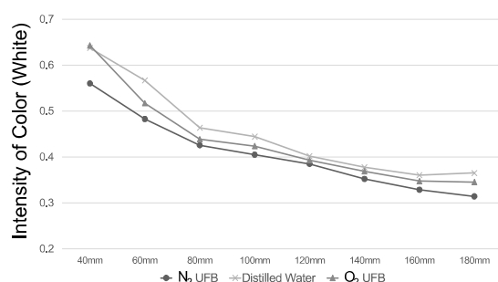
Fig. 4 Dependence of color intensity (Normalized with white) on distance from spray nozzle by ImageJ software.
