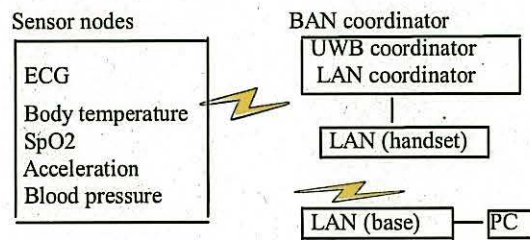
Fig.1 UWB BAN Experimental System
